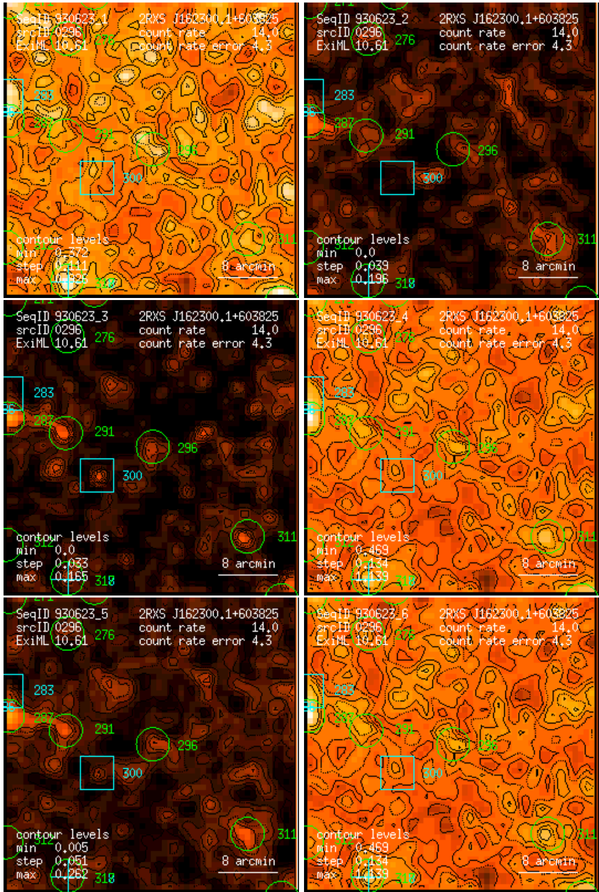
Figure 296: RASS 930623: detection 0296: band rate images, Gaussian filter: (1) PSPC channels 11 – 41, (2) 52 – 90, (3) 91 – 201, (4) 11 – 235, (5) 52 – 201, (6) 11 – 201. Broad band rates in counts/ks. Band rate contour levels in counts/ks/arcmin 2 .
