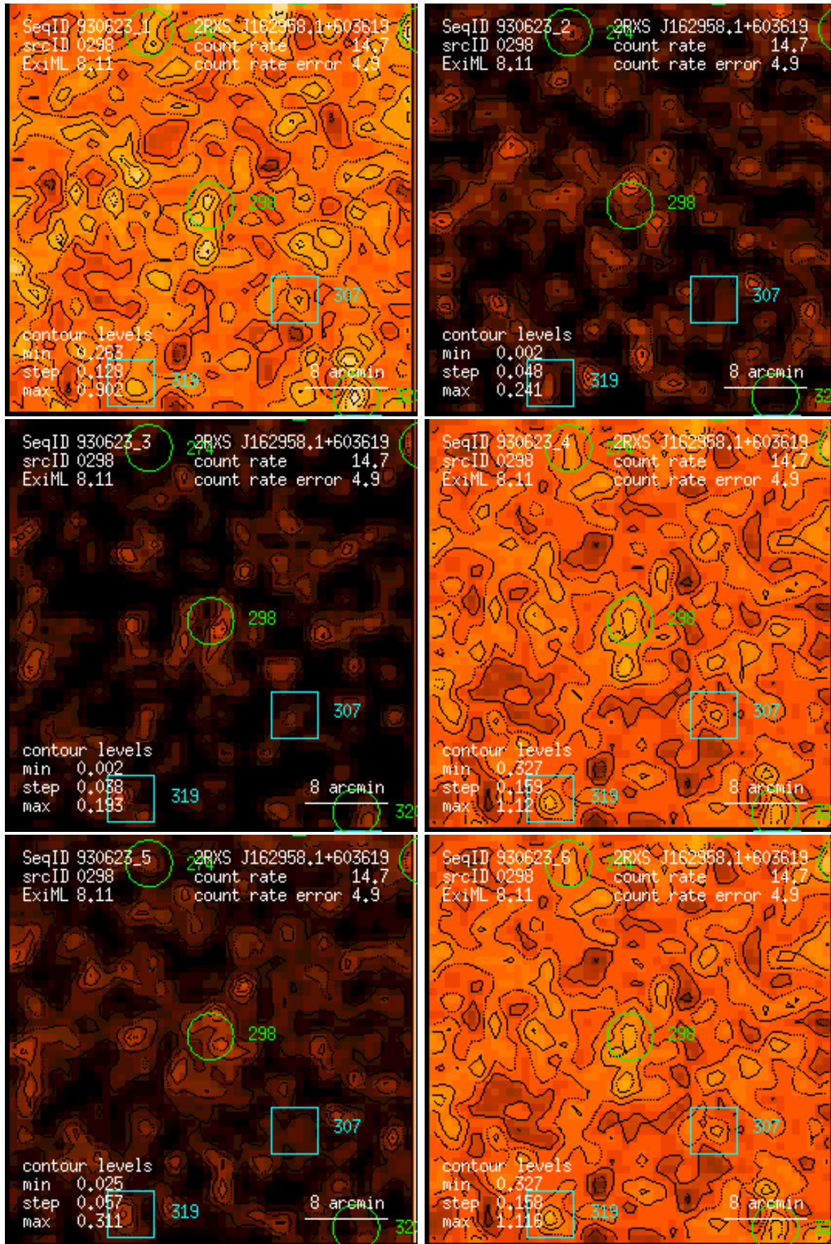
Figure 298: RASS 930623: detection 0298: band rate images, Gaussian filter: (1) PSPC channels 11 – 41, (2) 52 – 90, (3) 91 – 201, (4) 11 – 235, (5) 52 – 201, (6) 11 – 201. Broad band rates in counts/ks. Band rate contour levels in counts/ks/arcmin 2 .
