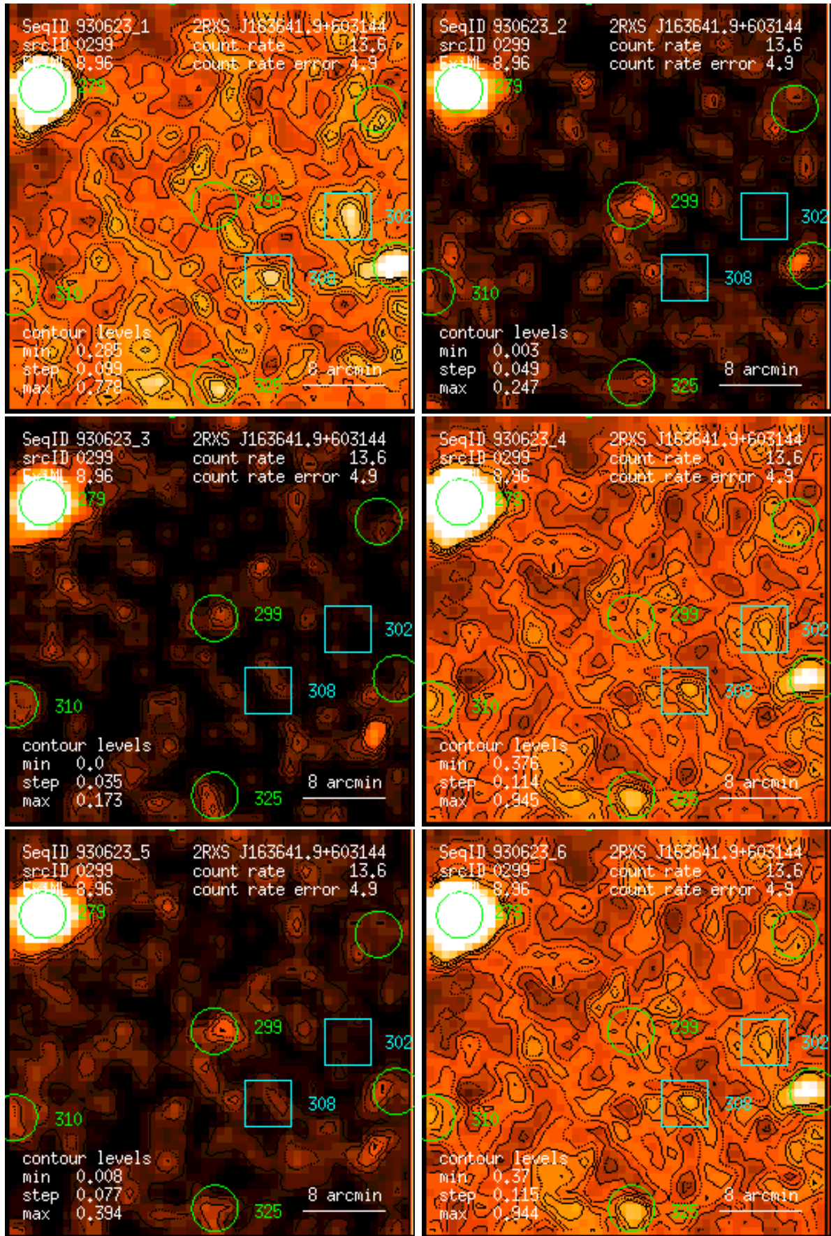
Figure 299: RASS 930623: detection 0299: band rate images, Gaussian filter: (1) PSPC channels 11 – 41, (2) 52 – 90, (3) 91 – 201, (4) 11 – 235, (5) 52 – 201, (6) 11 – 201. Broad band rates in counts/ks. Band rate contour levels in counts/ks/arcmin 2 .
