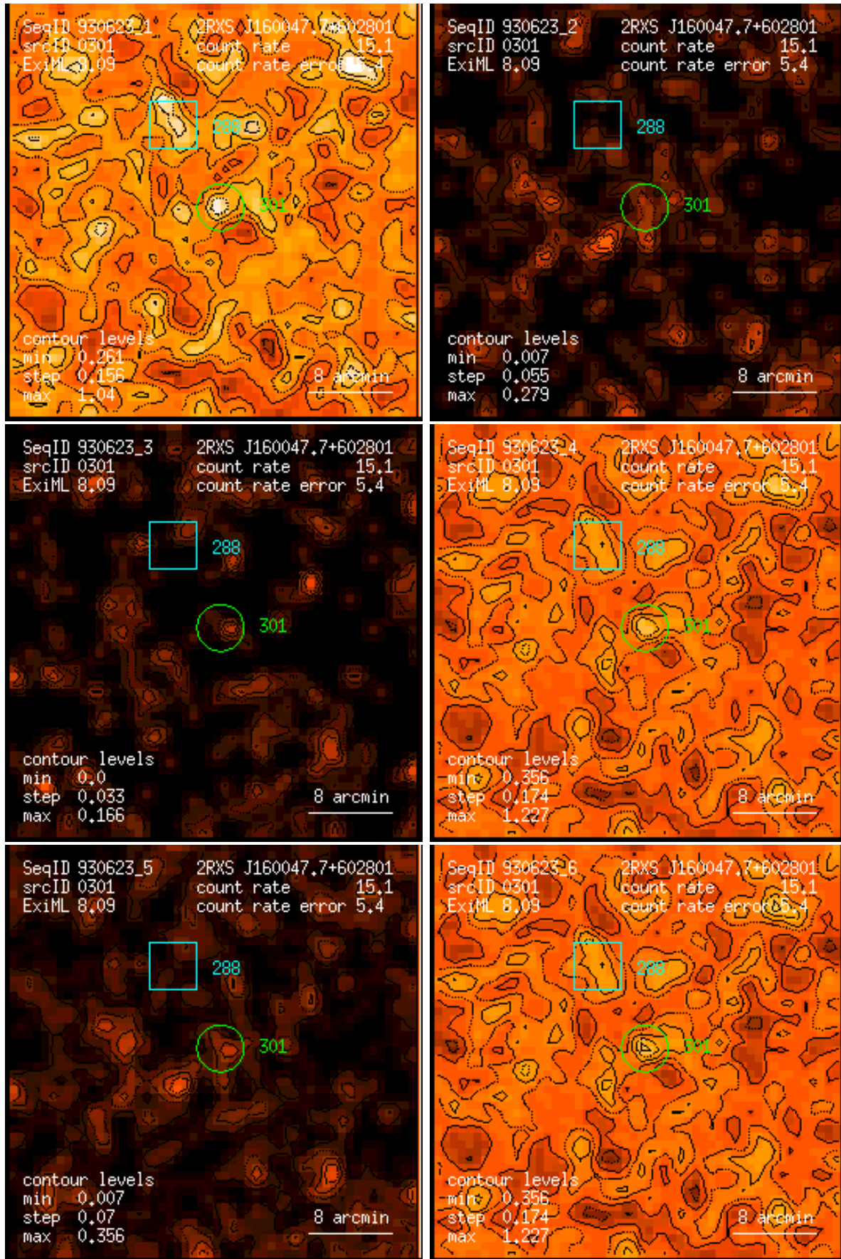
Figure 301: RASS 930623: detection 0301: band rate images, Gaussian filter: (1) PSPC channels 11 – 41, (2) 52 – 90, (3) 91 – 201, (4) 11 – 235, (5) 52 – 201, (6) 11 – 201. Broad band rates in counts/ks. Band rate contour levels in counts/ks/arcmin 2 .
