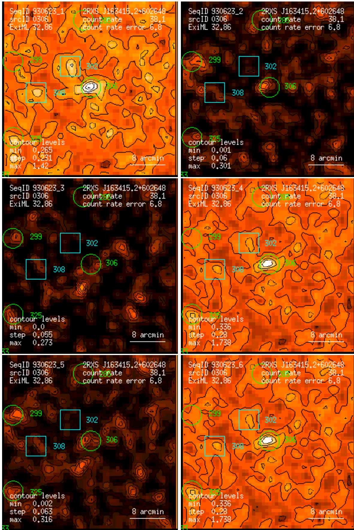
Figure 306: RASS 930623: detection 0306: band rate images, Gaussian filter: (1) PSPC channels 11 – 41, (2) 52 – 90, (3) 91 – 201, (4) 11 – 235, (5) 52 – 201, (6) 11 – 201. Broad band rates in counts/ks. Band rate contour levels in counts/ks/arcmin 2 .
