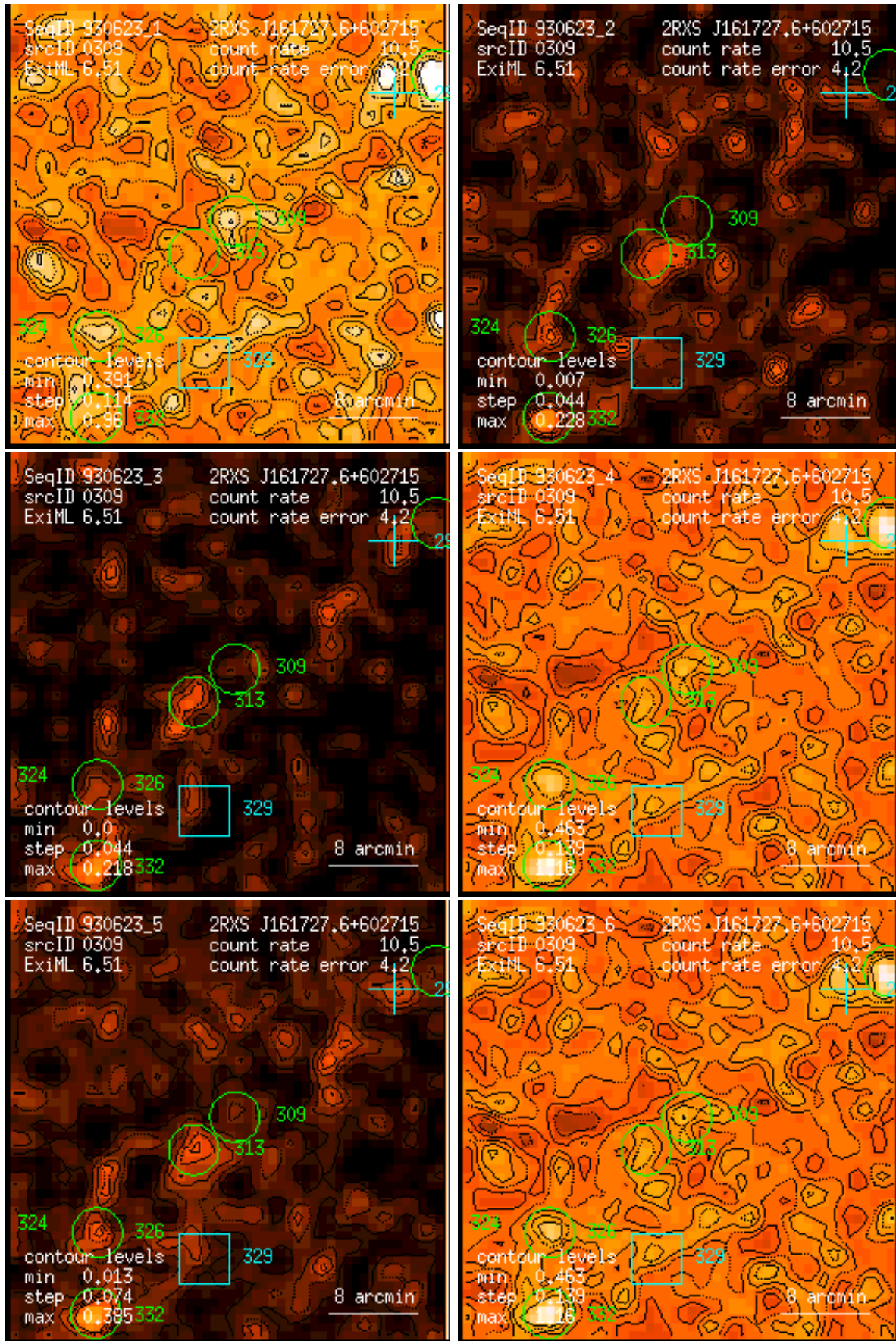
Figure 309: RASS 930623: detection 0309: band rate images, Gaussian filter: (1) PSPC channels 11 – 41, (2) 52 – 90, (3) 91 – 201, (4) 11 – 235, (5) 52 – 201, (6) 11 – 201. Broad band rates in counts/ks. Band rate contour levels in counts/ks/arcmin 2 .
