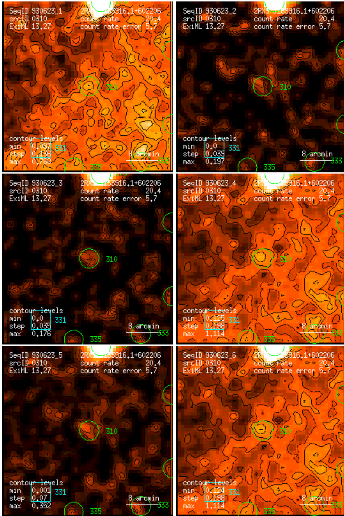
Figure 310: RASS 930623: detection 0310: band rate images, Gaussian filter: (1) PSPC channels 11 – 41, (2) 52 – 90, (3) 91 – 201, (4) 11 – 235, (5) 52 – 201, (6) 11 – 201. Broad band rates in counts/ks. Band rate contour levels in counts/ks/arcmin 2 .
