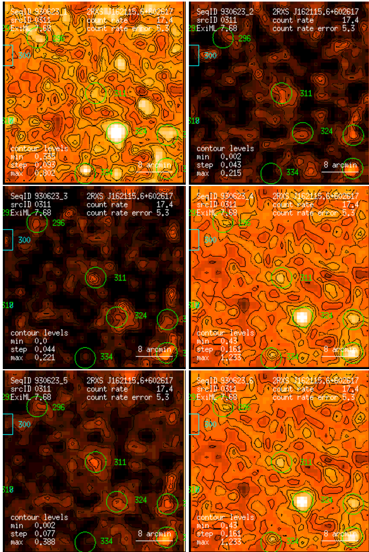
Figure 311: RASS 930623: detection 0311: band rate images, Gaussian filter: (1) PSPC channels 11 – 41, (2) 52 – 90, (3) 91 – 201, (4) 11 – 235, (5) 52 – 201, (6) 11 – 201. Broad band rates in counts/ks. Band rate contour levels in counts/ks/arcmin 2 .
