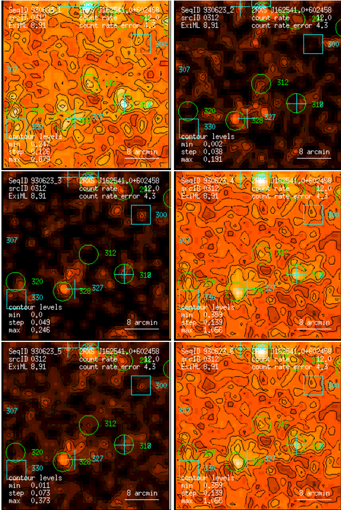
Figure 312: RASS 930623: detection 0312: band rate images, Gaussian filter: (1) PSPC channels 11 – 41, (2) 52 – 90, (3) 91 – 201, (4) 11 – 235, (5) 52 – 201, (6) 11 – 201. Broad band rates in counts/ks. Band rate contour levels in counts/ks/arcmin 2 .
