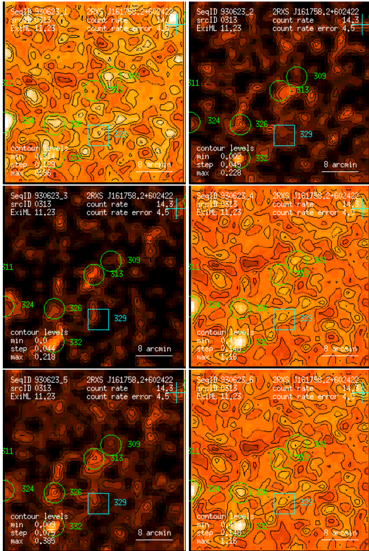
Figure 313: RASS 930623: detection 0313: band rate images, Gaussian filter: (1) PSPC channels 11 – 41, (2) 52 – 90, (3) 91 – 201, (4) 11 – 235, (5) 52 – 201, (6) 11 – 201. Broad band rates in counts/ks. Band rate contour levels in counts/ks/arcmin 2 .
