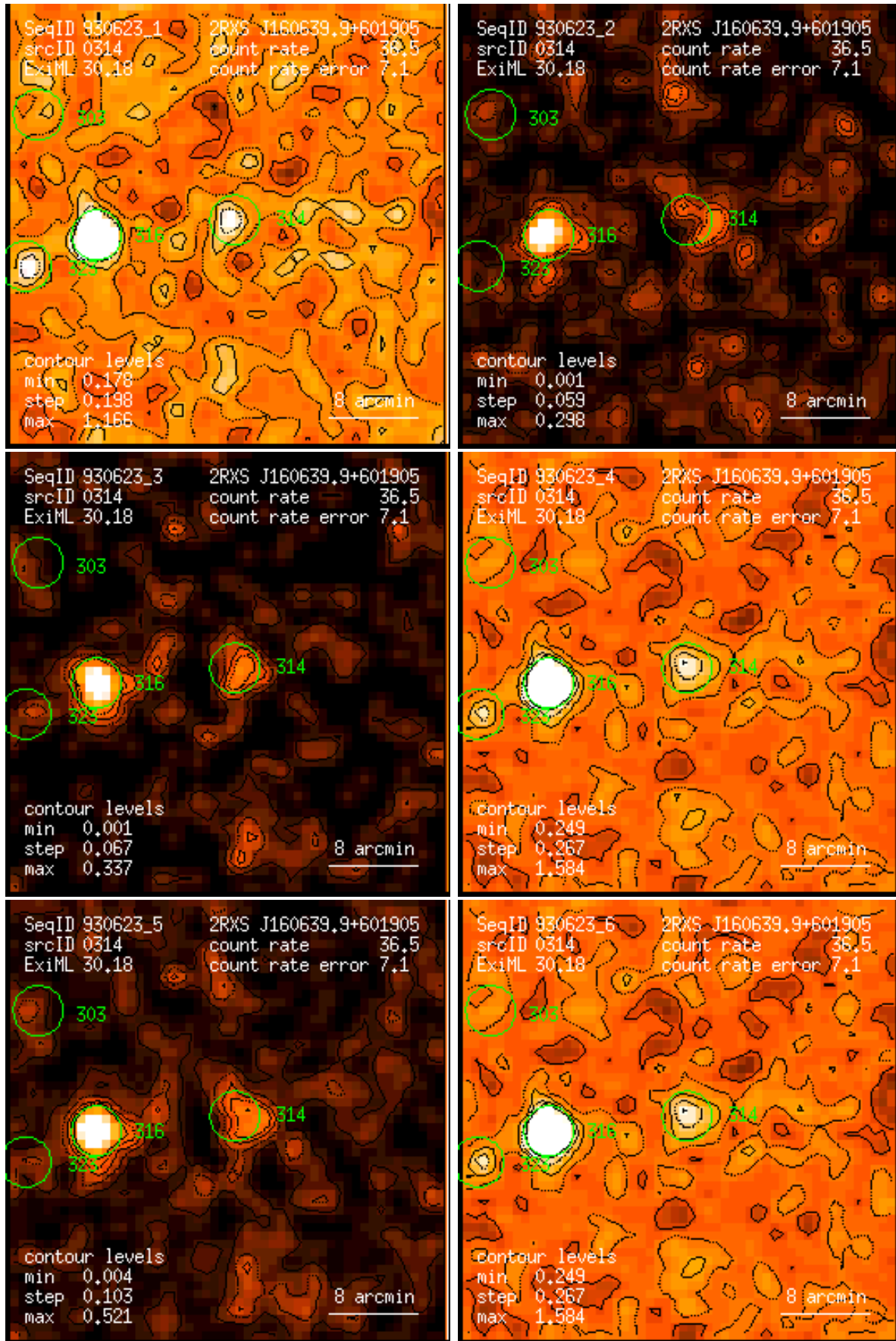
Figure 314: RASS 930623: detection 0314: band rate images, Gaussian filter: (1) PSPC channels 11 – 41, (2) 52 – 90, (3) 91 – 201, (4) 11 – 235, (5) 52 – 201, (6) 11 – 201. Broad band rates in counts/ks. Band rate contour levels in counts/ks/arcmin 2 .
