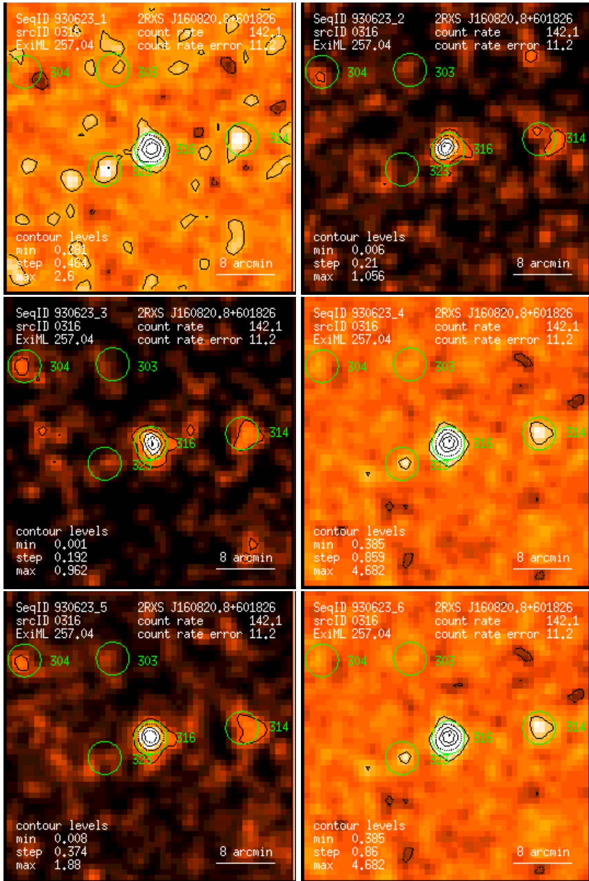
Figure 316: RASS 930623: detection 0316: band rate images, Gaussian filter: (1) PSPC channels 11 – 41, (2) 52 – 90, (3) 91 – 201, (4) 11 – 235, (5) 52 – 201, (6) 11 – 201. Broad band rates in counts/ks. Band rate contour levels in counts/ks/arcmin 2 .
