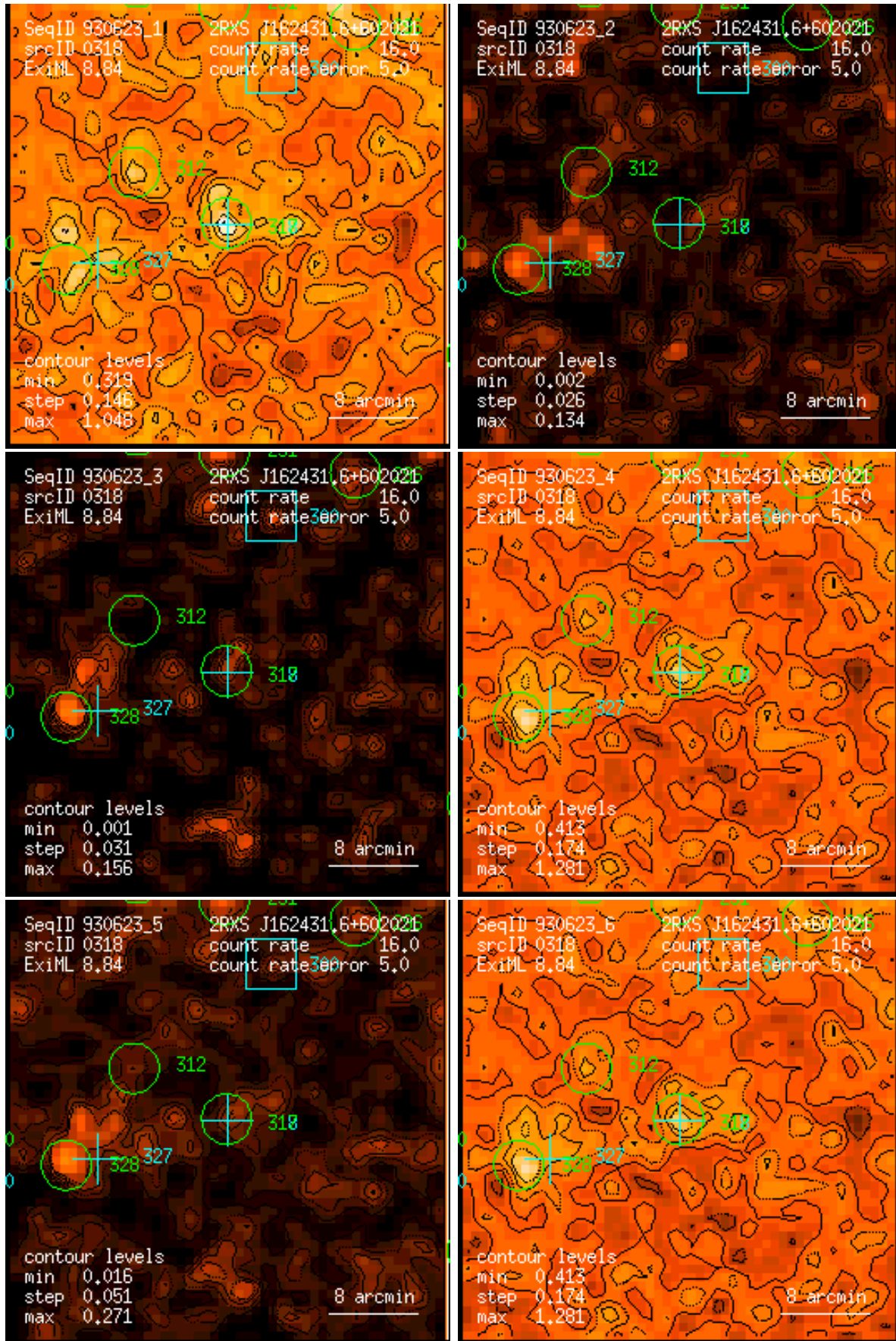
Figure 318: RASS 930623: detection 0318: band rate images, Gaussian filter: (1) PSPC channels 11 – 41, (2) 52 – 90, (3) 91 – 201, (4) 11 – 235, (5) 52 – 201, (6) 11 – 201. Broad band rates in counts/ks. Band rate contour levels in counts/ks/arcmin 2 .
