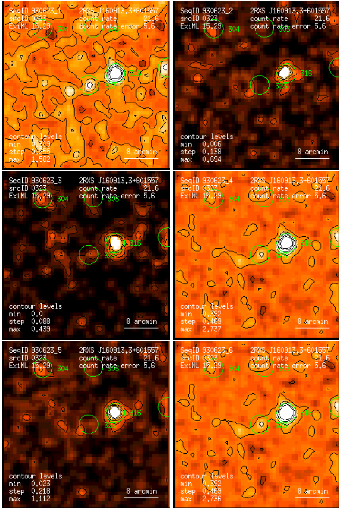
Figure 323: RASS 930623: detection 0323: band rate images, Gaussian filter: (1) PSPC channels 11 – 41, (2) 52 – 90, (3) 91 – 201, (4) 11 – 235, (5) 52 – 201, (6) 11 – 201. Broad band rates in counts/ks. Band rate contour levels in counts/ks/arcmin 2 .
