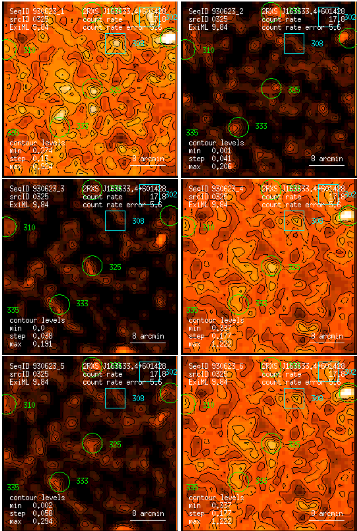
Figure 325: RASS 930623: detection 0325: band rate images, Gaussian filter: (1) PSPC channels 11 – 41, (2) 52 – 90, (3) 91 – 201, (4) 11 – 235, (5) 52 – 201, (6) 11 – 201. Broad band rates in counts/ks. Band rate contour levels in counts/ks/arcmin 2 .
