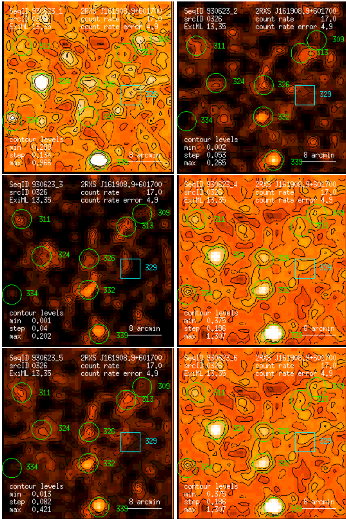
Figure 326: RASS 930623: detection 0326: band rate images, Gaussian filter: (1) PSPC channels 11 – 41, (2) 52 – 90, (3) 91 – 201, (4) 11 – 235, (5) 52 – 201, (6) 11 – 201. Broad band rates in counts/ks. Band rate contour levels in counts/ks/arcmin 2 .
