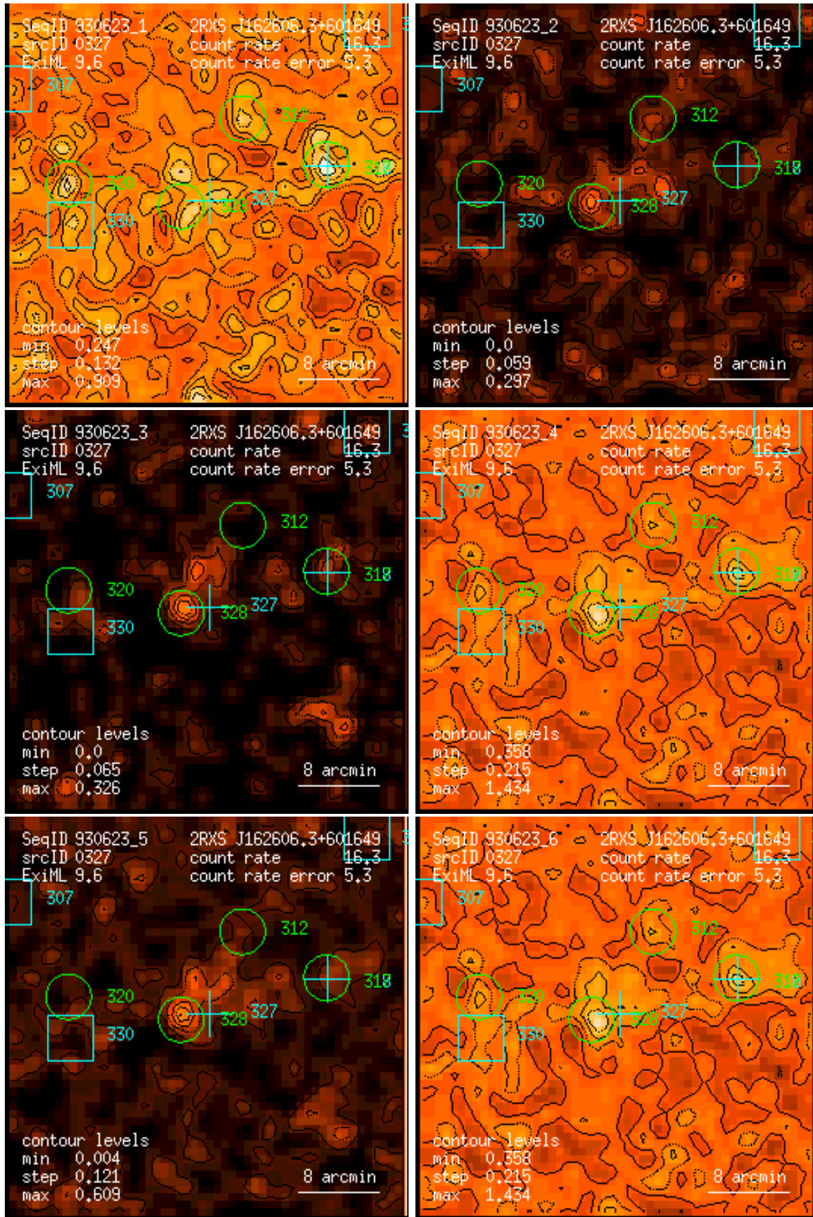
Figure 327: RASS 930623: detection 0327: band rate images, Gaussian filter: (1) PSPC channels 11 – 41, (2) 52 – 90, (3) 91 – 201, (4) 11 – 235, (5) 52 – 201, (6) 11 – 201. Broad band rates in counts/ks. Band rate contour levels in counts/ks/arcmin 2 .
