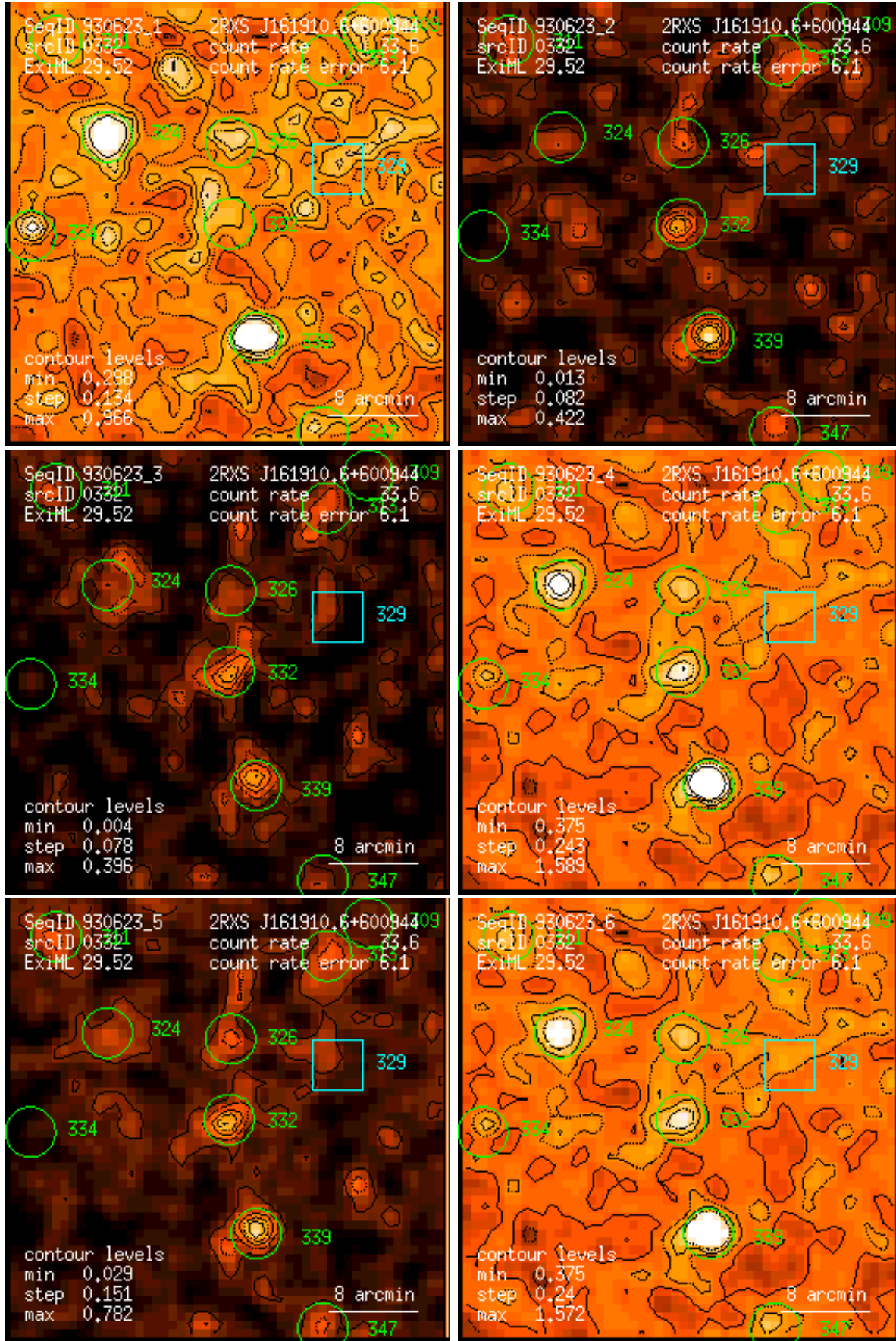
Figure 332: RASS 930623: detection 0332: band rate images, Gaussian filter: (1) PSPC channels 11 – 41, (2) 52 – 90, (3) 91 – 201, (4) 11 – 235, (5) 52 – 201, (6) 11 – 201. Broad band rates in counts/ks. Band rate contour levels in counts/ks/arcmin 2 .
