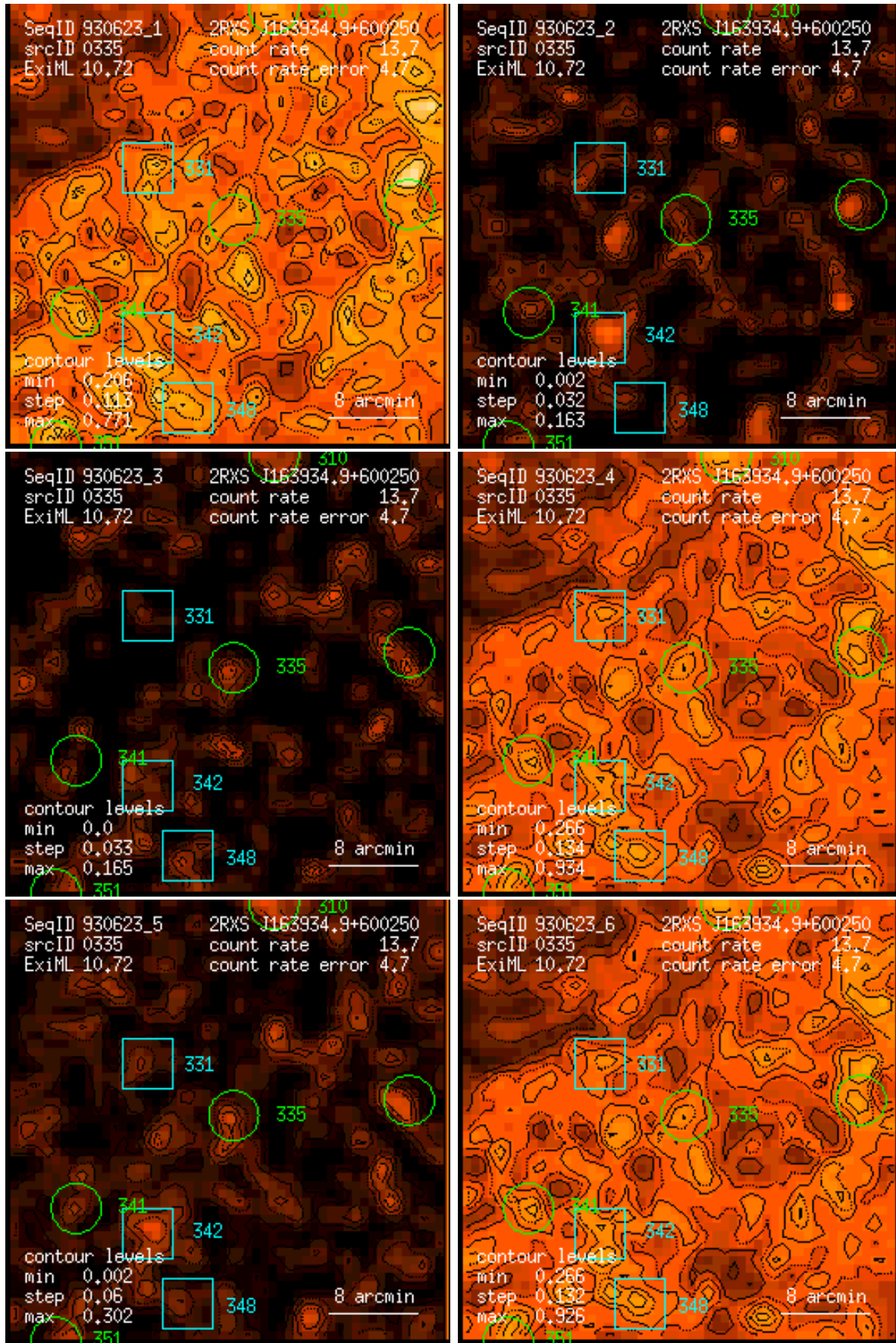
Figure 335: RASS 930623: detection 0335: band rate images, Gaussian filter: (1) PSPC channels 11 – 41, (2) 52 – 90, (3) 91 – 201, (4) 11 – 235, (5) 52 – 201, (6) 11 – 201. Broad band rates in counts/ks. Band rate contour levels in counts/ks/arcmin 2 .
