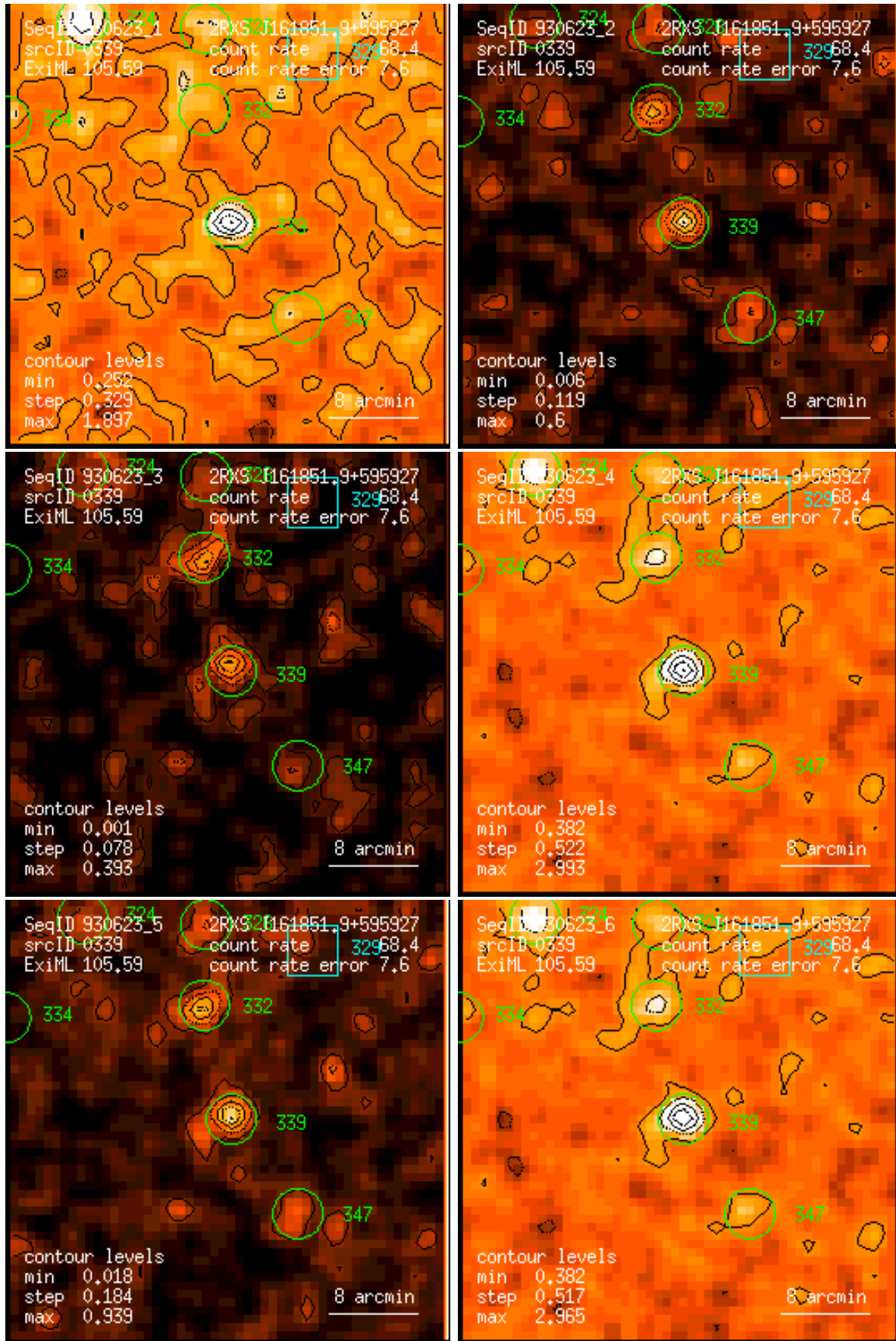
Figure 339: RASS 930623: detection 0339: band rate images, Gaussian filter: (1) PSPC channels 11 – 41, (2) 52 – 90, (3) 91 – 201, (4) 11 – 235, (5) 52 – 201, (6) 11 – 201. Broad band rates in counts/ks. Band rate contour levels in counts/ks/arcmin 2 .
