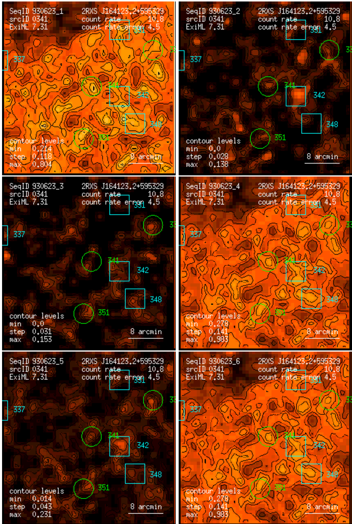
Figure 341: RASS 930623: detection 0341: band rate images, Gaussian filter: (1) PSPC channels 11 – 41, (2) 52 – 90, (3) 91 – 201, (4) 11 – 235, (5) 52 – 201, (6) 11 – 201. Broad band rates in counts/ks. Band rate contour levels in counts/ks/arcmin 2 .
