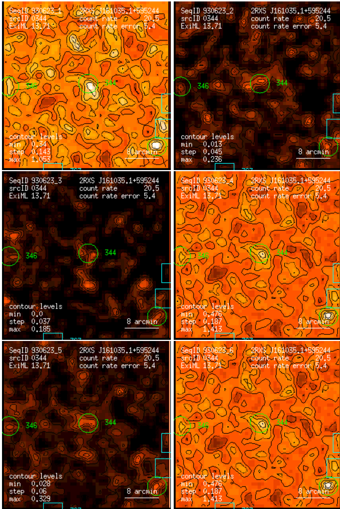
Figure 344: RASS 930623: detection 0344: band rate images, Gaussian filter: (1) PSPC channels 11 – 41, (2) 52 – 90, (3) 91 – 201, (4) 11 – 235, (5) 52 – 201, (6) 11 – 201. Broad band rates in counts/ks. Band rate contour levels in counts/ks/arcmin 2 .
