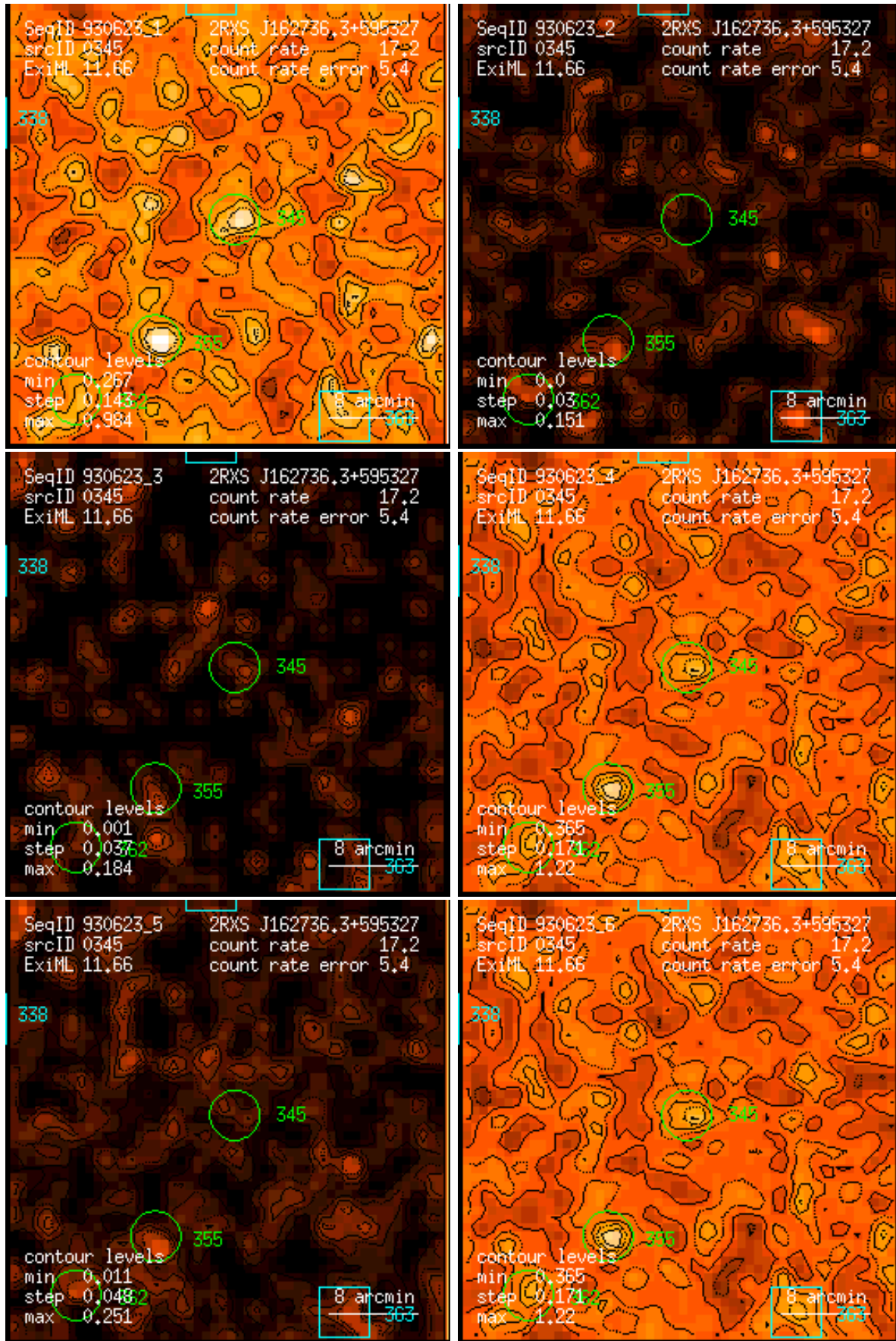
Figure 345: RASS 930623: detection 0345: band rate images, Gaussian filter: (1) PSPC channels 11 – 41, (2) 52 – 90, (3) 91 – 201, (4) 11 – 235, (5) 52 – 201, (6) 11 – 201. Broad band rates in counts/ks. Band rate contour levels in counts/ks/arcmin 2 .
