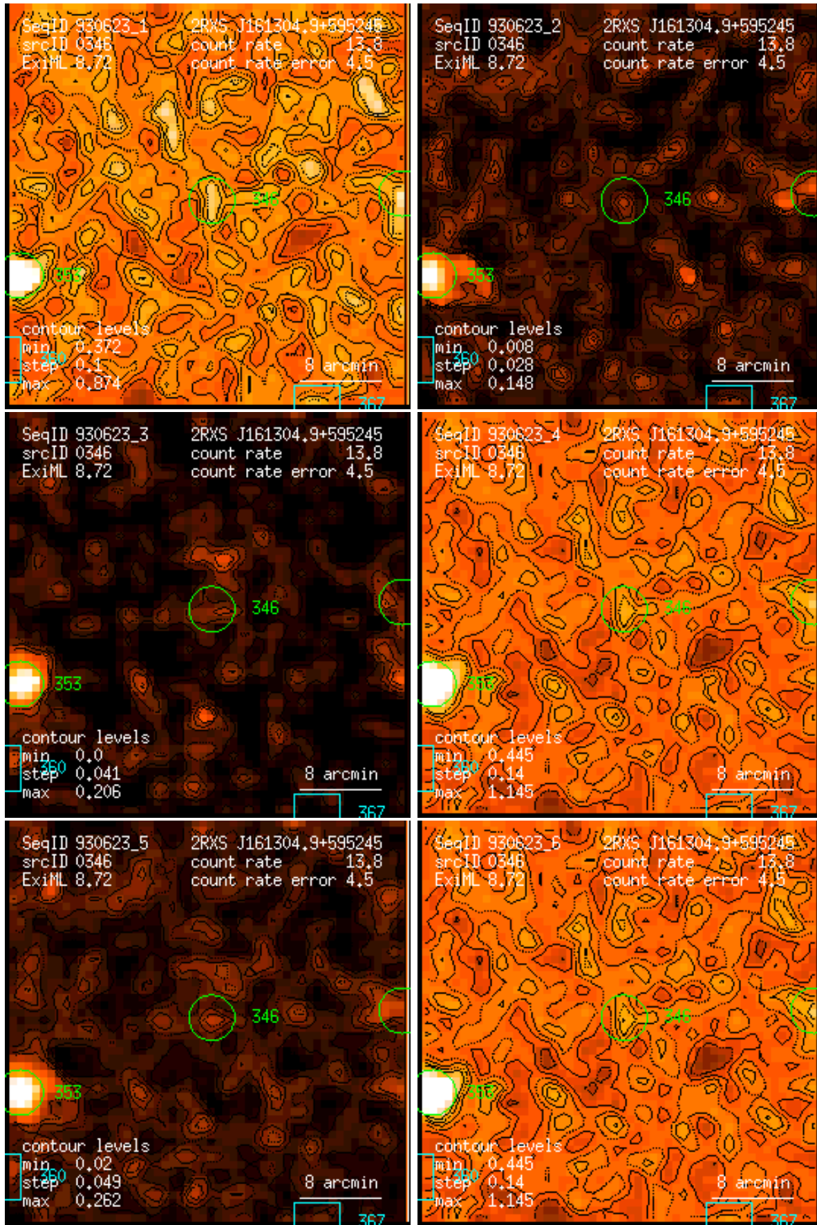
Figure 346: RASS 930623: detection 0346: band rate images, Gaussian filter: (1) PSPC channels 11 – 41, (2) 52 – 90, (3) 91 – 201, (4) 11 – 235, (5) 52 – 201, (6) 11 – 201. Broad band rates in counts/ks. Band rate contour levels in counts/ks/arcmin 2 .
