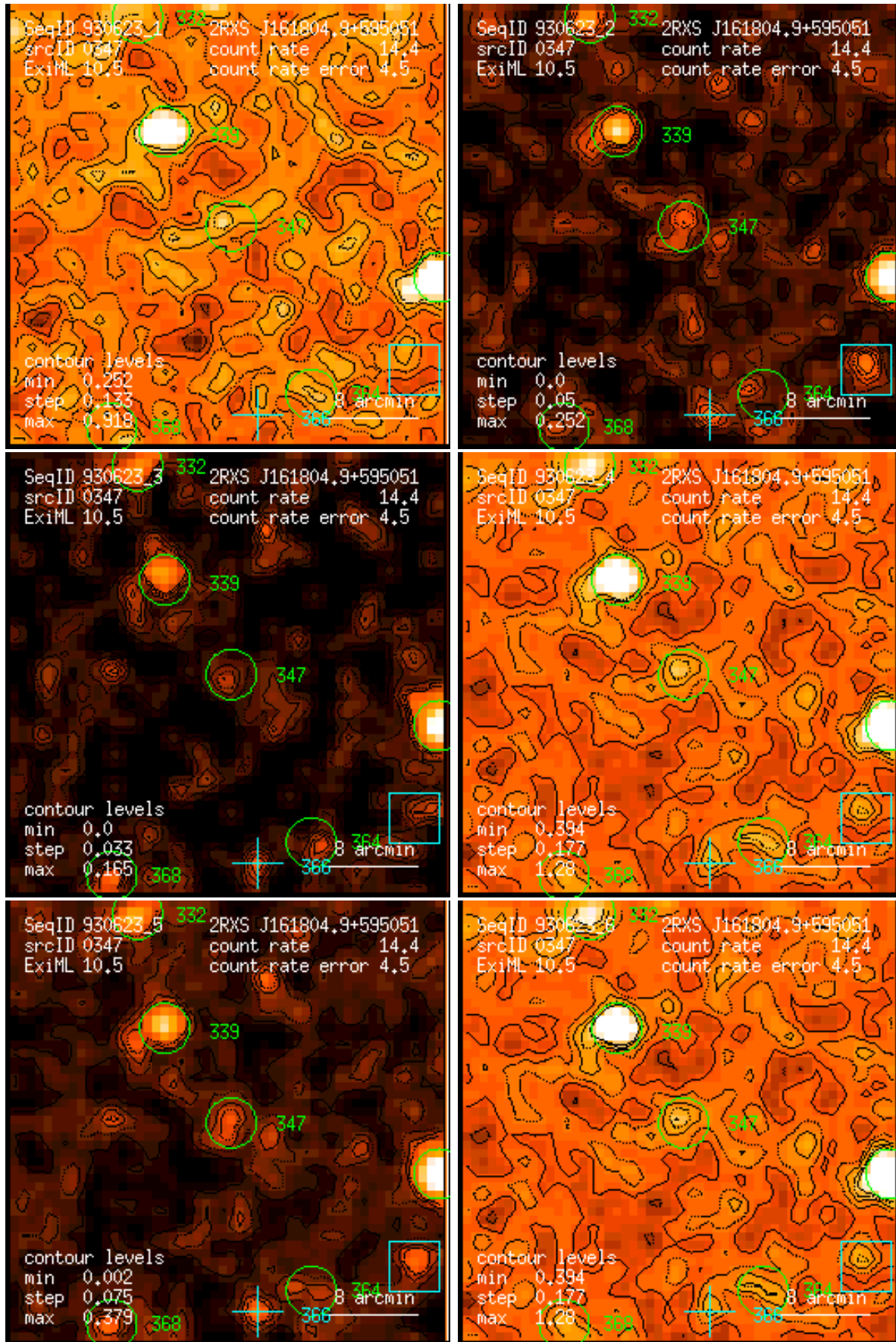
Figure 347: RASS 930623: detection 0347: band rate images, Gaussian filter: (1) PSPC channels 11 – 41, (2) 52 – 90, (3) 91 – 201, (4) 11 – 235, (5) 52 – 201, (6) 11 – 201. Broad band rates in counts/ks. Band rate contour levels in counts/ks/arcmin 2 .
