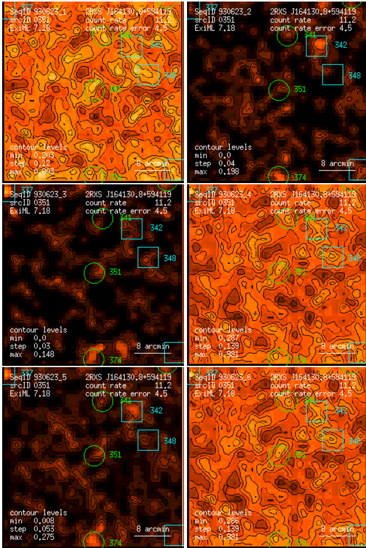
Figure 351: RASS 930623: detection 0351: band rate images, Gaussian filter: (1) PSPC channels 11 – 41, (2) 52 – 90, (3) 91 – 201, (4) 11 – 235, (5) 52 – 201, (6) 11 – 201. Broad band rates in counts/ks. Band rate contour levels in counts/ks/arcmin 2 .
