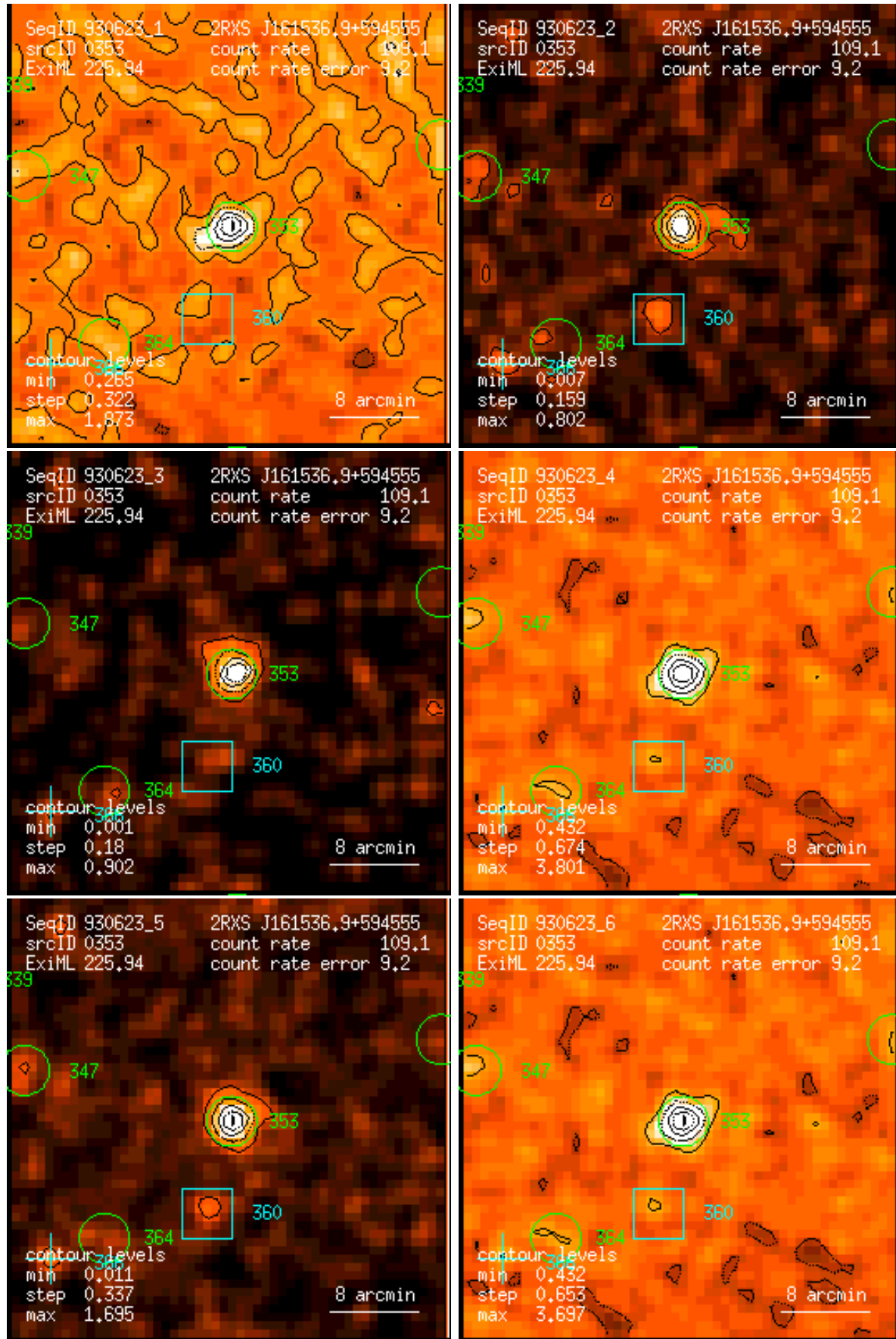
Figure 353: RASS 930623: detection 0353: band rate images, Gaussian filter: (1) PSPC channels 11 – 41, (2) 52 – 90, (3) 91 – 201, (4) 11 – 235, (5) 52 – 201, (6) 11 – 201. Broad band rates in counts/ks. Band rate contour levels in counts/ks/arcmin 2 .
