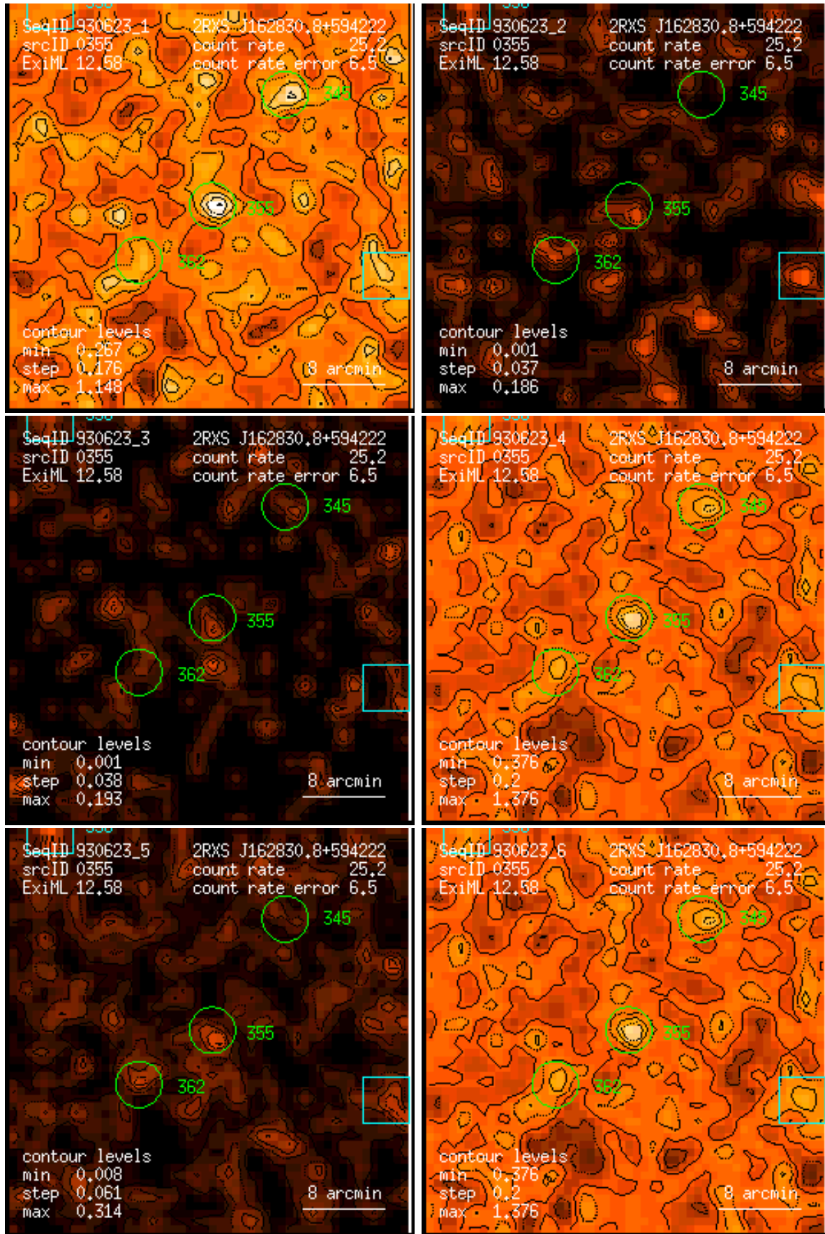
Figure 355: RASS 930623: detection 0355: band rate images, Gaussian filter: (1) PSPC channels 11 – 41, (2) 52 – 90, (3) 91 – 201, (4) 11 – 235, (5) 52 – 201, (6) 11 – 201. Broad band rates in counts/ks. Band rate contour levels in counts/ks/arcmin 2 .
