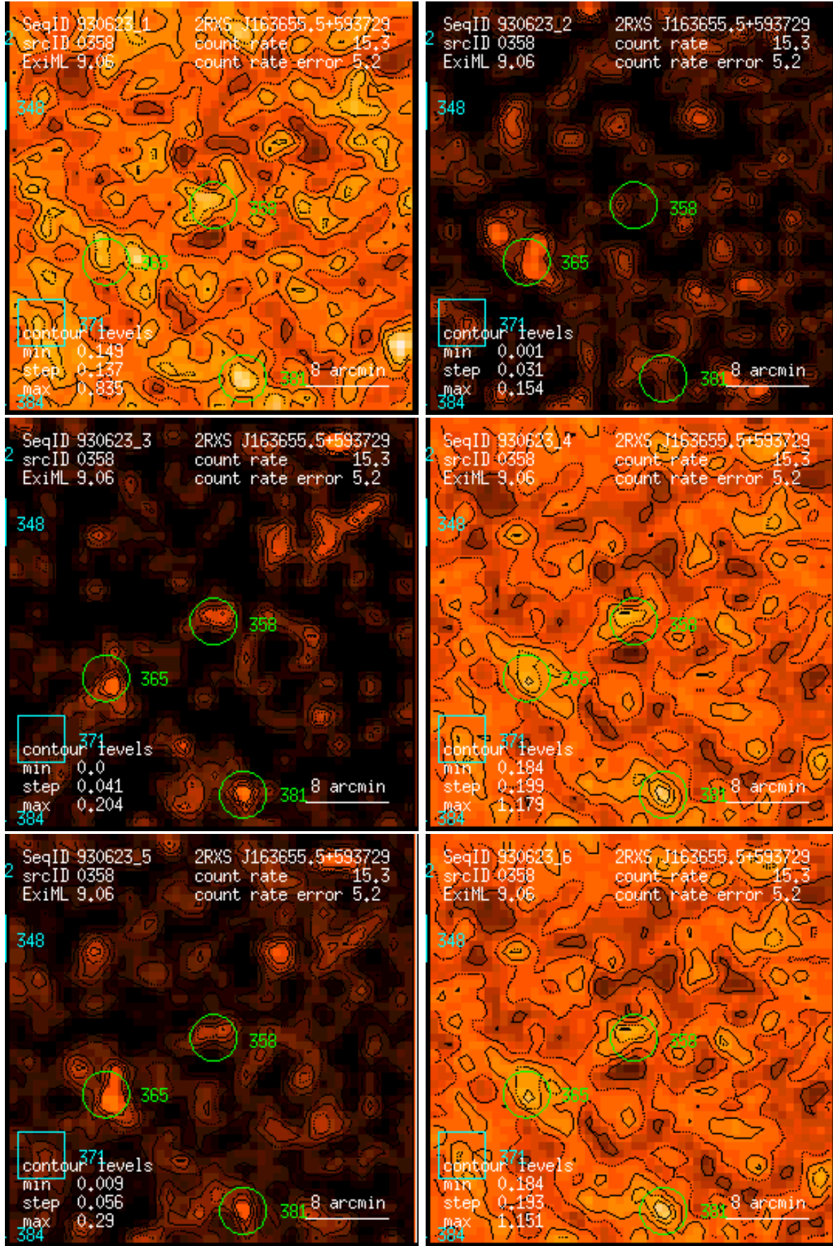
Figure 358: RASS 930623: detection 0358: band rate images, Gaussian filter: (1) PSPC channels 11 – 41, (2) 52 – 90, (3) 91 – 201, (4) 11 – 235, (5) 52 – 201, (6) 11 – 201. Broad band rates in counts/ks. Band rate contour levels in counts/ks/arcmin 2 .
