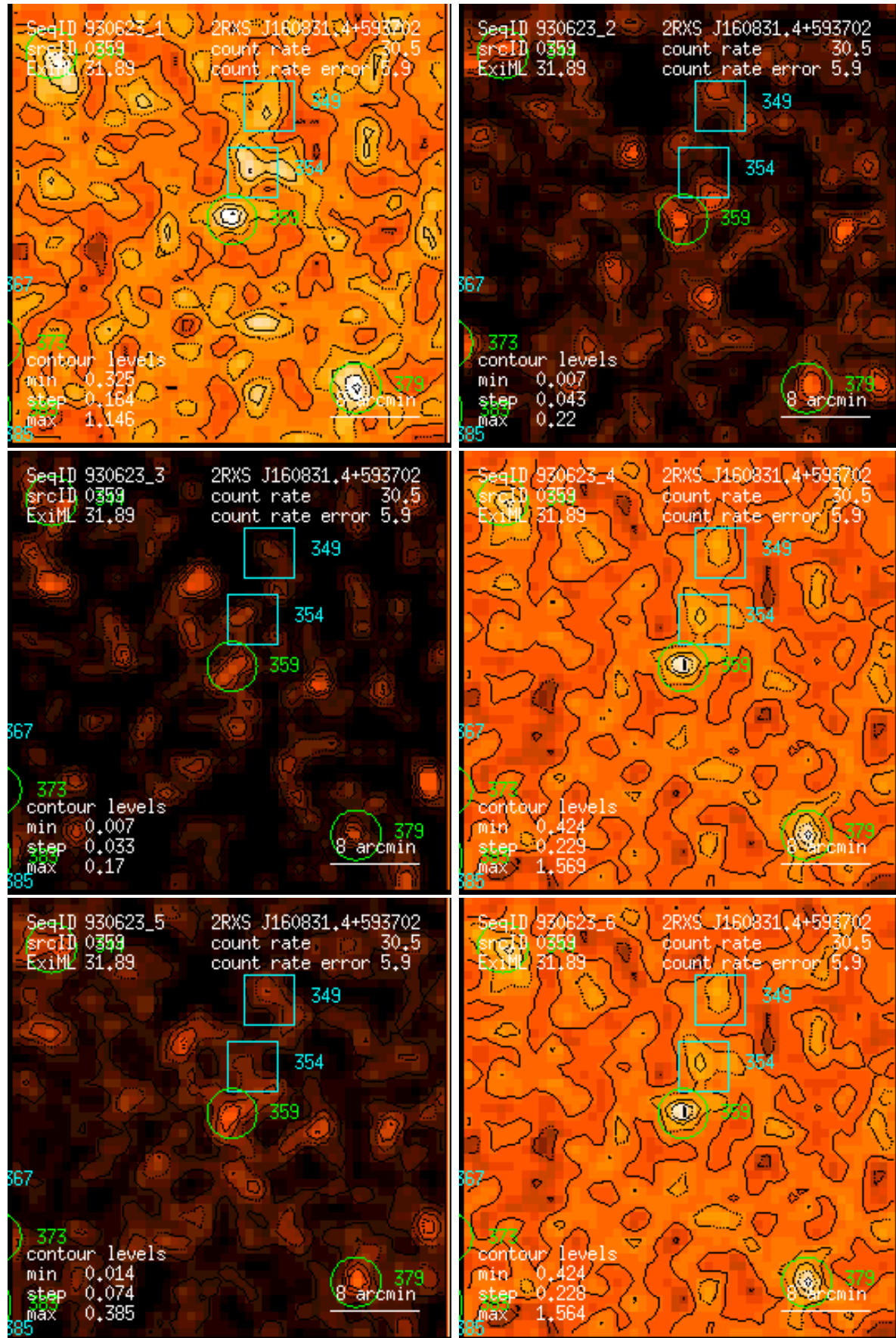
Figure 359: RASS 930623: detection 0359: band rate images, Gaussian filter: (1) PSPC channels 11 – 41, (2) 52 – 90, (3) 91 – 201, (4) 11 – 235, (5) 52 – 201, (6) 11 – 201. Broad band rates in counts/ks. Band rate contour levels in counts/ks/arcmin 2 .
