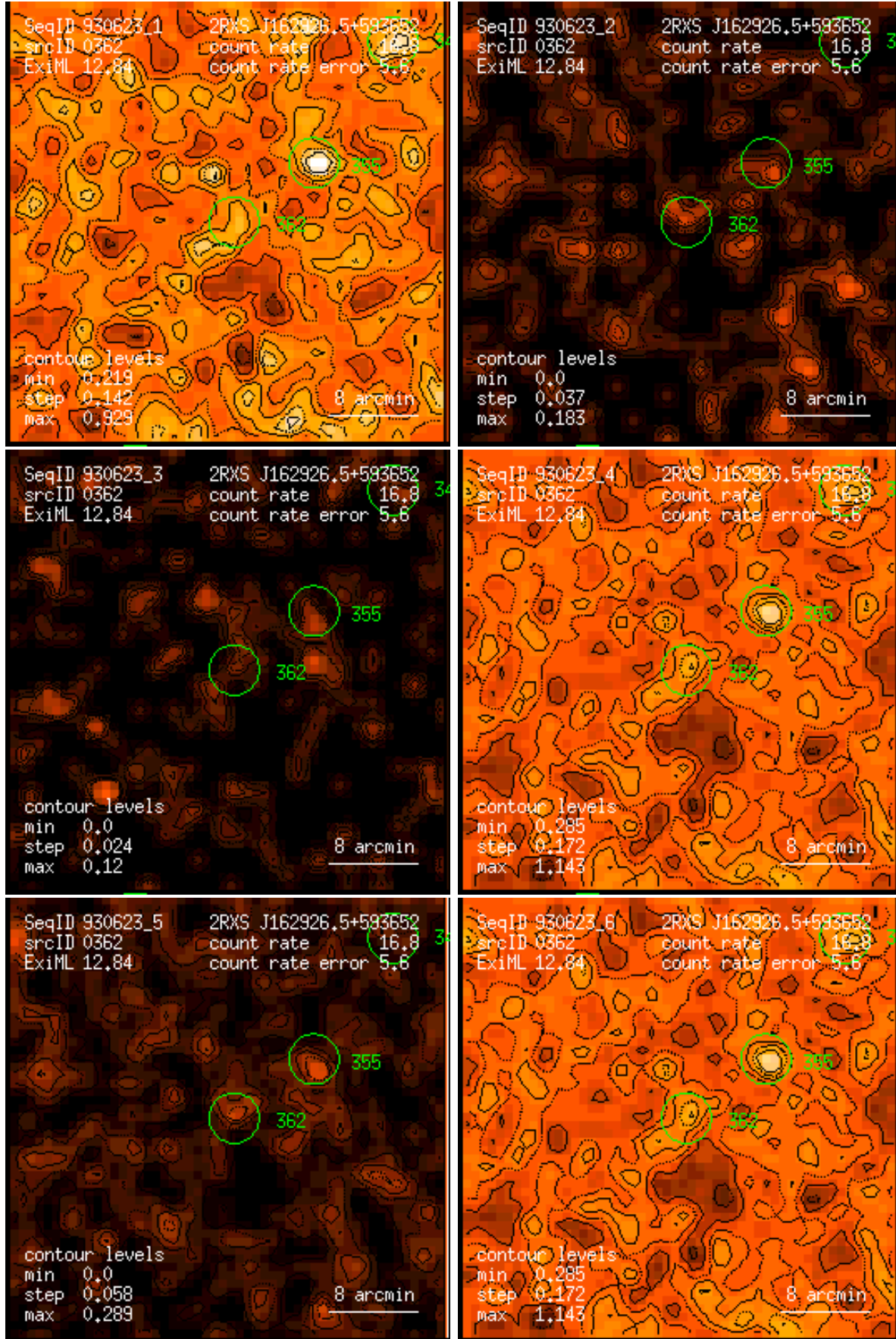
Figure 362: RASS 930623: detection 0362: band rate images, Gaussian filter: (1) PSPC channels 11 – 41, (2) 52 – 90, (3) 91 – 201, (4) 11 – 235, (5) 52 – 201, (6) 11 – 201. Broad band rates in counts/ks. Band rate contour levels in counts/ks/arcmin 2 .
