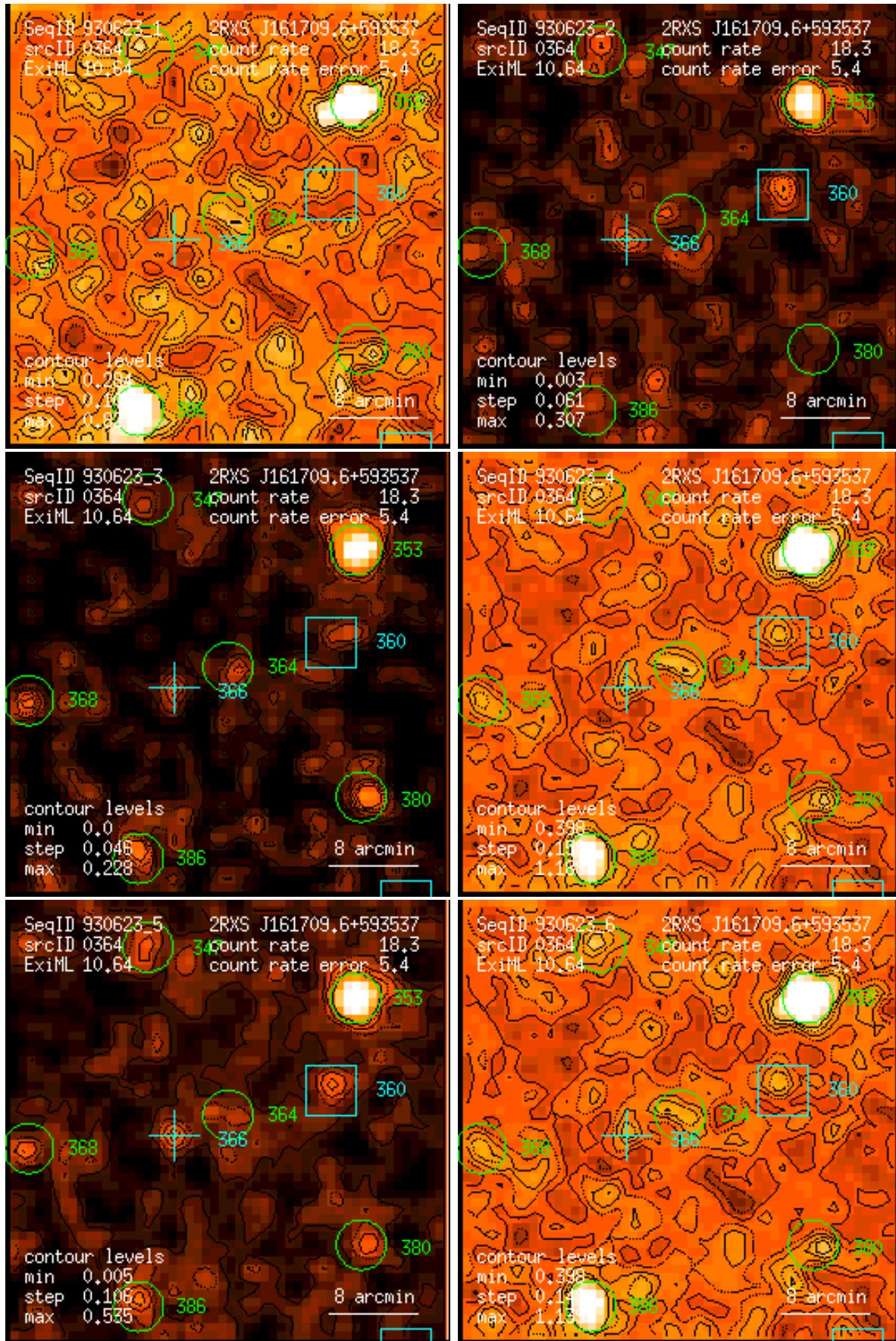
Figure 364: RASS 930623: detection 0364: band rate images, Gaussian filter: (1) PSPC channels 11 – 41, (2) 52 – 90, (3) 91 – 201, (4) 11 – 235, (5) 52 – 201, (6) 11 – 201. Broad band rates in counts/ks. Band rate contour levels in counts/ks/arcmin 2 .
