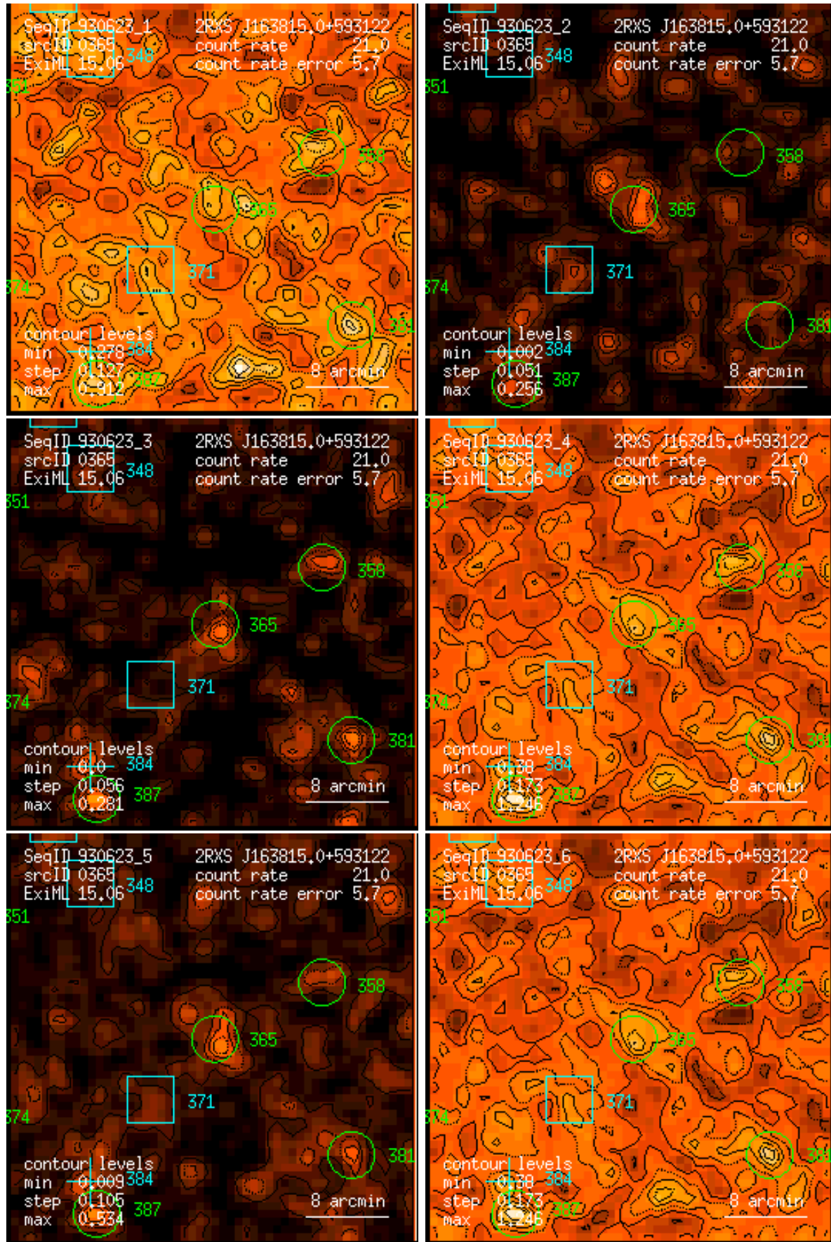
Figure 365: RASS 930623: detection 0365: band rate images, Gaussian filter: (1) PSPC channels 11 – 41, (2) 52 – 90, (3) 91 – 201, (4) 11 – 235, (5) 52 – 201, (6) 11 – 201. Broad band rates in counts/ks. Band rate contour levels in counts/ks/arcmin 2 .
