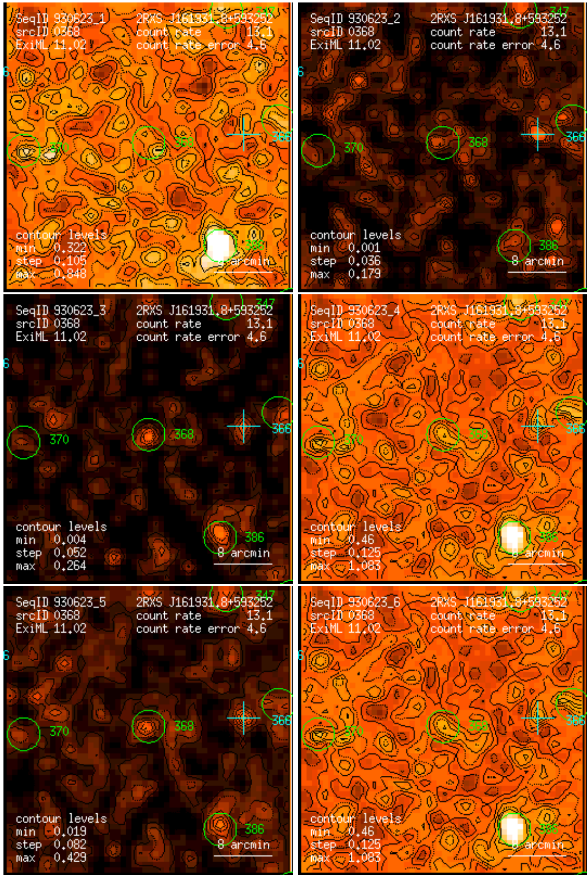
Figure 368: RASS 930623: detection 0368: band rate images, Gaussian filter: (1) PSPC channels 11 – 41, (2) 52 – 90, (3) 91 – 201, (4) 11 – 235, (5) 52 – 201, (6) 11 – 201. Broad band rates in counts/ks. Band rate contour levels in counts/ks/arcmin 2 .
