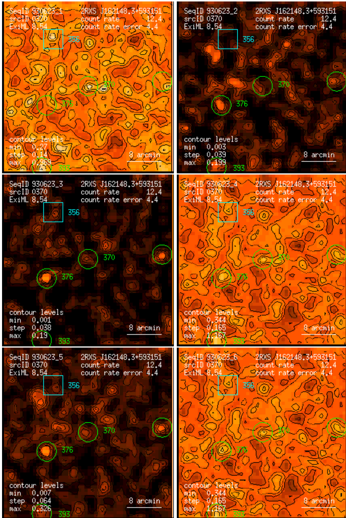
Figure 370: RASS 930623: detection 0370: band rate images, Gaussian filter: (1) PSPC channels 11 – 41, (2) 52 – 90, (3) 91 – 201, (4) 11 – 235, (5) 52 – 201, (6) 11 – 201. Broad band rates in counts/ks. Band rate contour levels in counts/ks/arcmin 2 .
