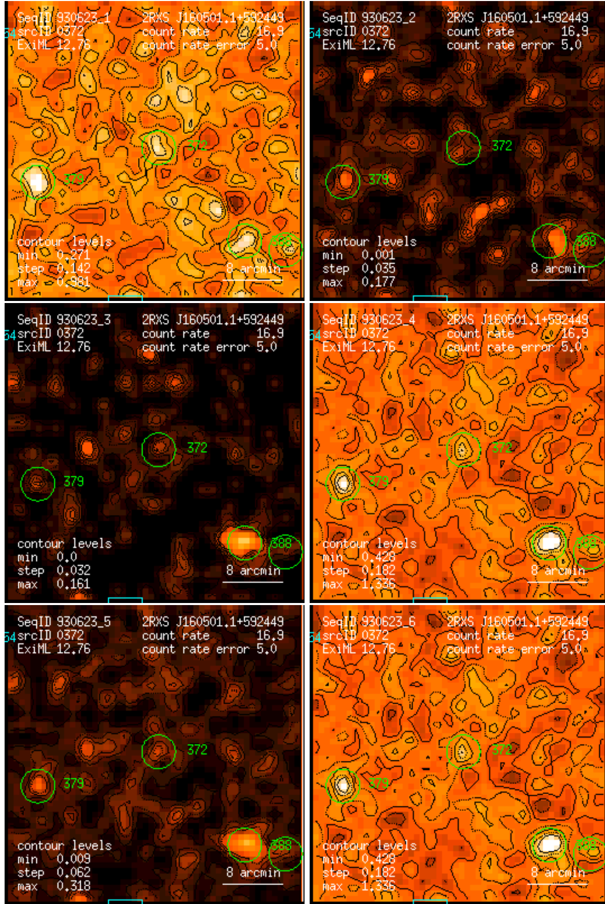
Figure 372: RASS 930623: detection 0372: band rate images, Gaussian filter: (1) PSPC channels 11 – 41, (2) 52 – 90, (3) 91 – 201, (4) 11 – 235, (5) 52 – 201, (6) 11 – 201. Broad band rates in counts/ks. Band rate contour levels in counts/ks/arcmin 2 .
