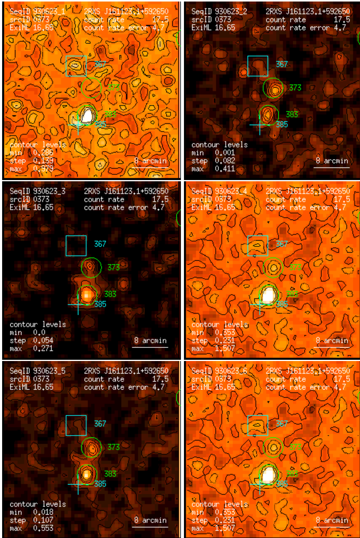
Figure 373: RASS 930623: detection 0373: band rate images, Gaussian filter: (1) PSPC channels 11 – 41, (2) 52 – 90, (3) 91 – 201, (4) 11 – 235, (5) 52 – 201, (6) 11 – 201. Broad band rates in counts/ks. Band rate contour levels in counts/ks/arcmin 2 .
