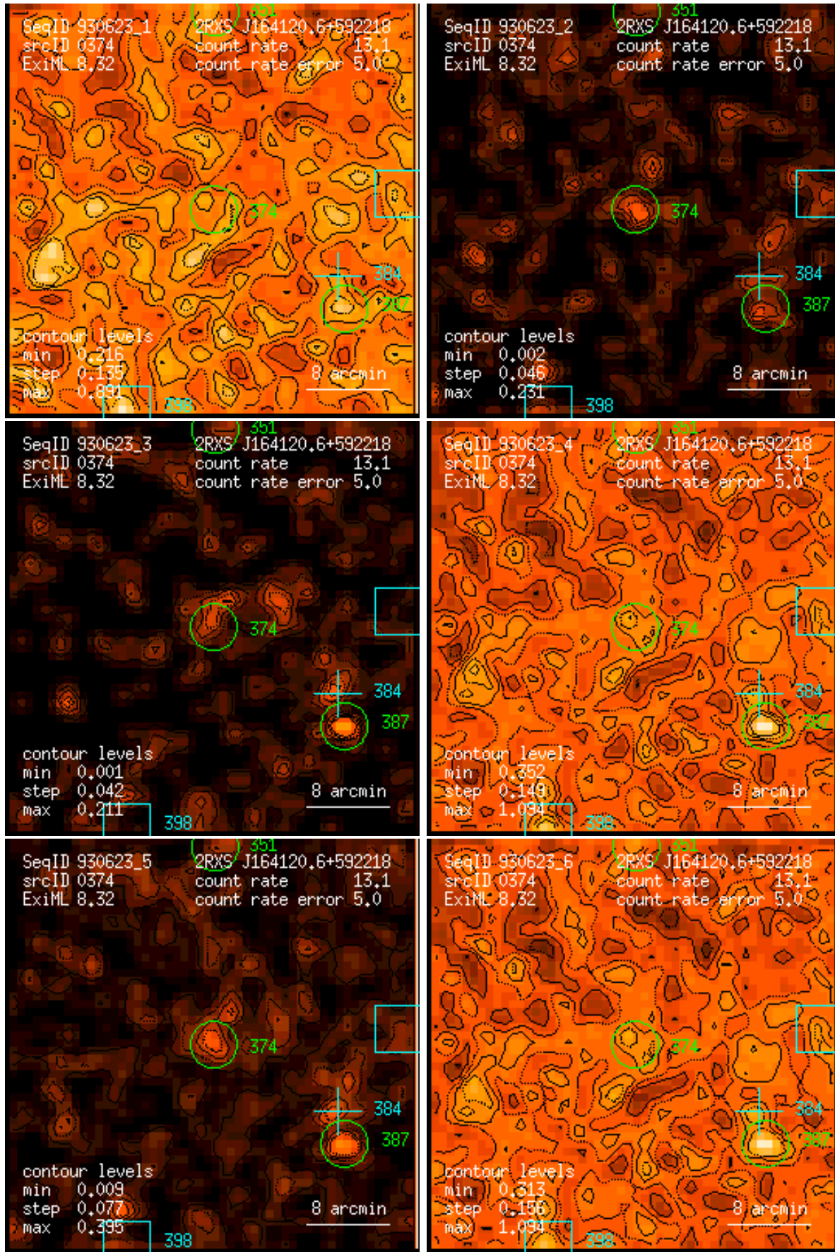
Figure 374: RASS 930623: detection 0374: band rate images, Gaussian filter: (1) PSPC channels 11 – 41, (2) 52 – 90, (3) 91 – 201, (4) 11 – 235, (5) 52 – 201, (6) 11 – 201. Broad band rates in counts/ks. Band rate contour levels in counts/ks/arcmin 2 .
