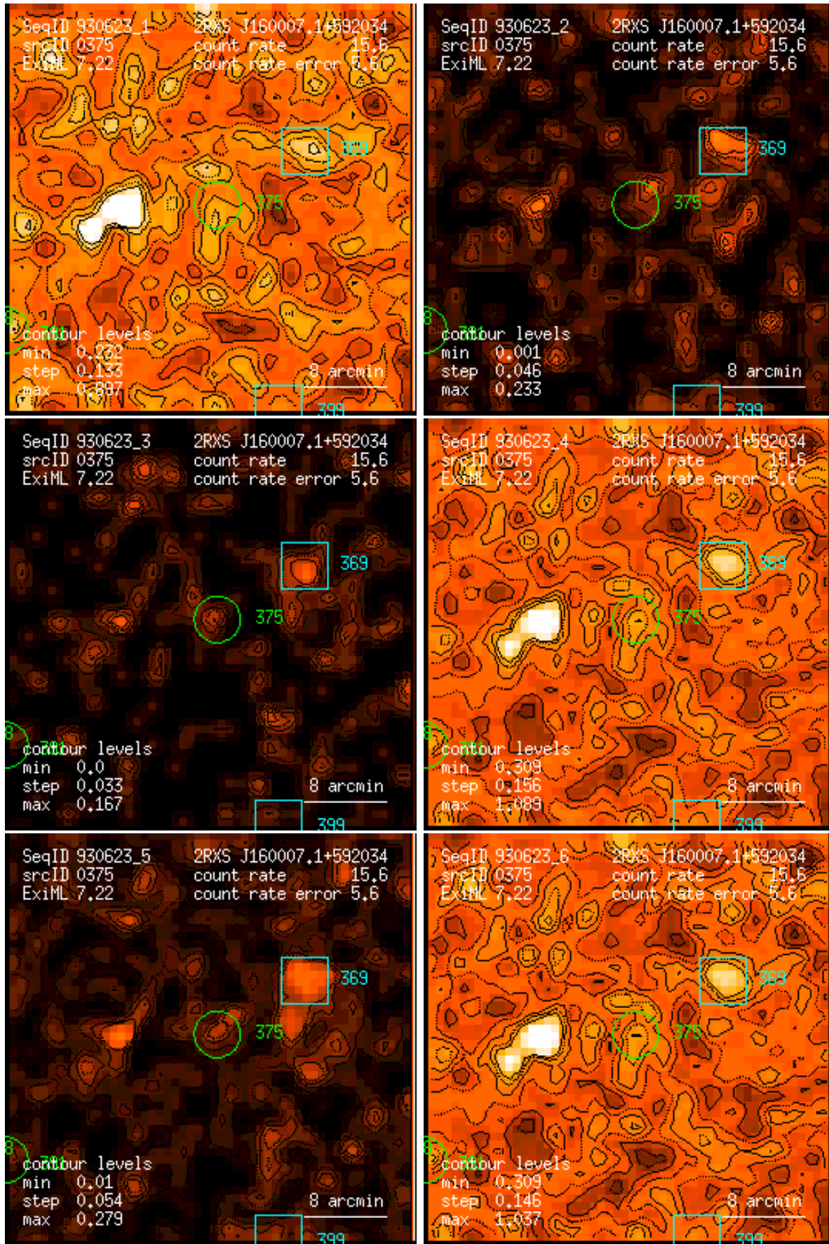
Figure 375: RASS 930623: detection 0375: band rate images, Gaussian filter: (1) PSPC channels 11 – 41, (2) 52 – 90, (3) 91 – 201, (4) 11 – 235, (5) 52 – 201, (6) 11 – 201. Broad band rates in counts/ks. Band rate contour levels in counts/ks/arcmin 2 .
