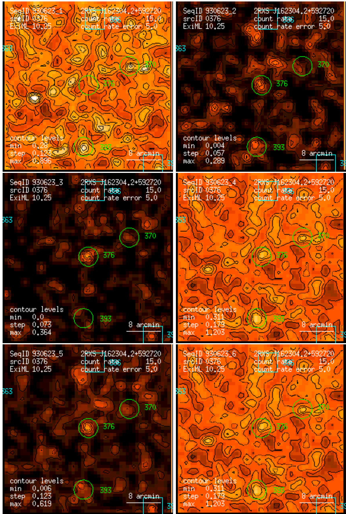
Figure 376: RASS 930623: detection 0376: band rate images, Gaussian filter: (1) PSPC channels 11 – 41, (2) 52 – 90, (3) 91 – 201, (4) 11 – 235, (5) 52 – 201, (6) 11 – 201. Broad band rates in counts/ks. Band rate contour levels in counts/ks/arcmin 2 .
