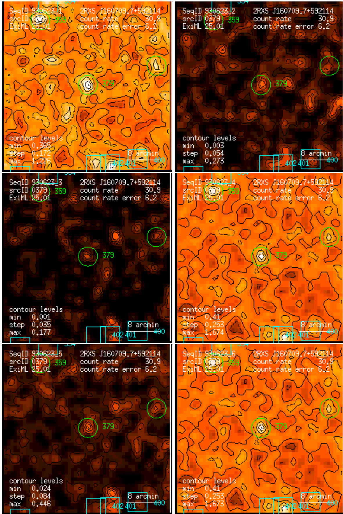
Figure 379: RASS 930623: detection 0379: band rate images, Gaussian filter: (1) PSPC channels 11 – 41, (2) 52 – 90, (3) 91 – 201, (4) 11 – 235, (5) 52 – 201, (6) 11 – 201. Broad band rates in counts/ks. Band rate contour levels in counts/ks/arcmin 2 .
