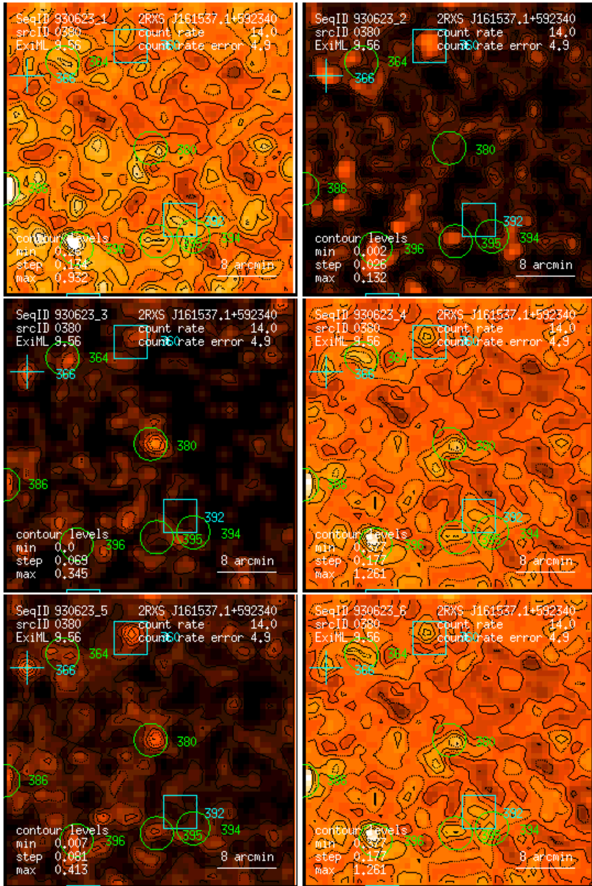
Figure 380: RASS 930623: detection 0380: band rate images, Gaussian filter: (1) PSPC channels 11 – 41, (2) 52 – 90, (3) 91 – 201, (4) 11 – 235, (5) 52 – 201, (6) 11 – 201. Broad band rates in counts/ks. Band rate contour levels in counts/ks/arcmin 2 .
