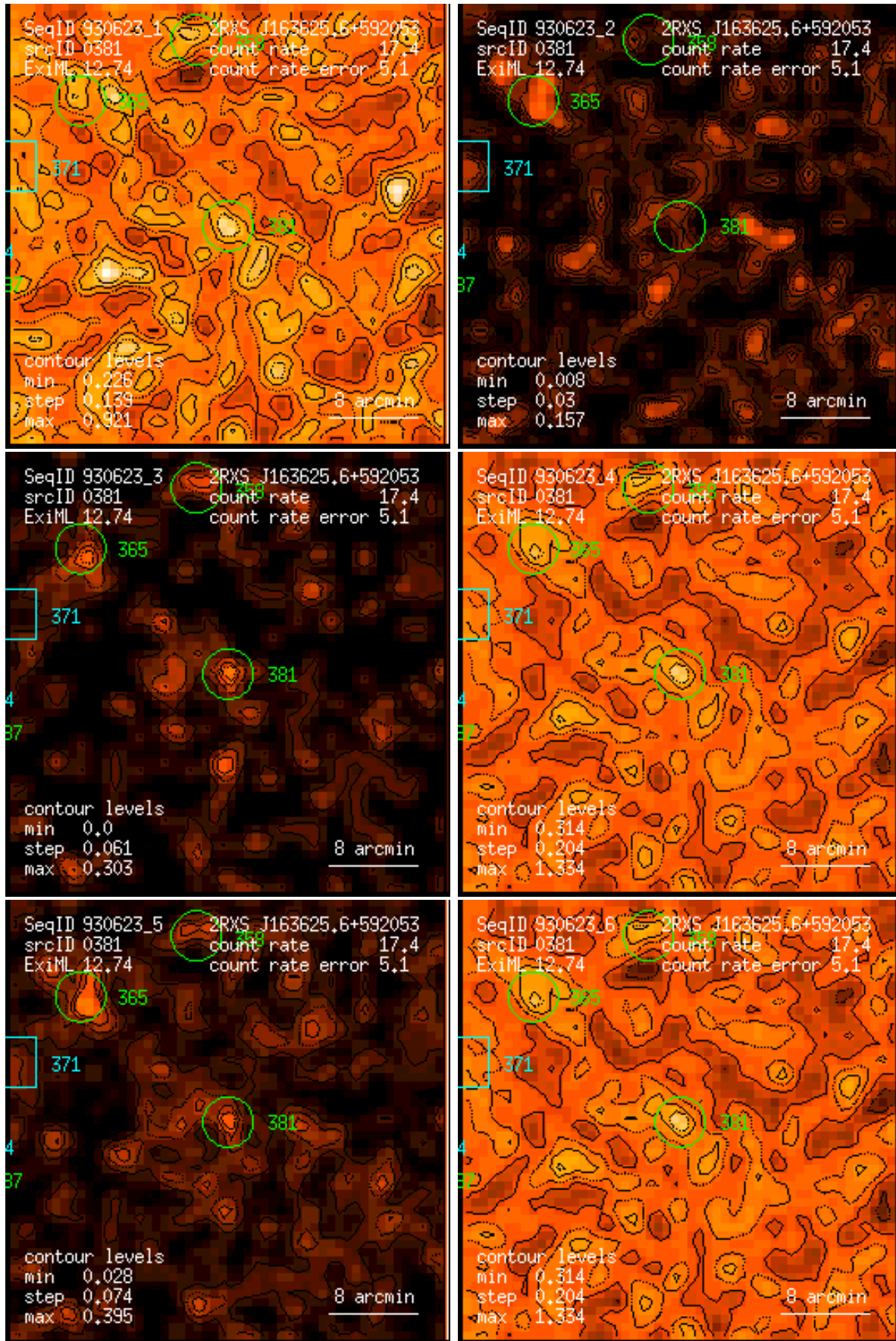
Figure 381: RASS 930623: detection 0381: band rate images, Gaussian filter: (1) PSPC channels 11 – 41, (2) 52 – 90, (3) 91 – 201, (4) 11 – 235, (5) 52 – 201, (6) 11 – 201. Broad band rates in counts/ks. Band rate contour levels in counts/ks/arcmin 2 .
