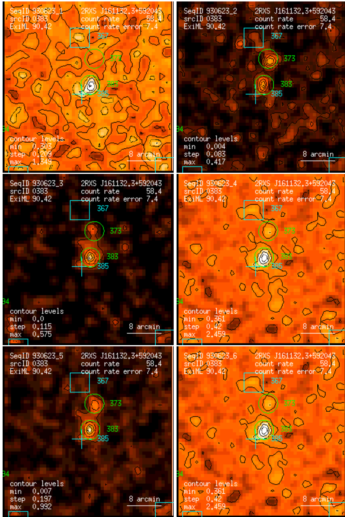
Figure 383: RASS 930623: detection 0383: band rate images, Gaussian filter: (1) PSPC channels 11 – 41, (2) 52 – 90, (3) 91 – 201, (4) 11 – 235, (5) 52 – 201, (6) 11 – 201. Broad band rates in counts/ks. Band rate contour levels in counts/ks/arcmin 2 .
