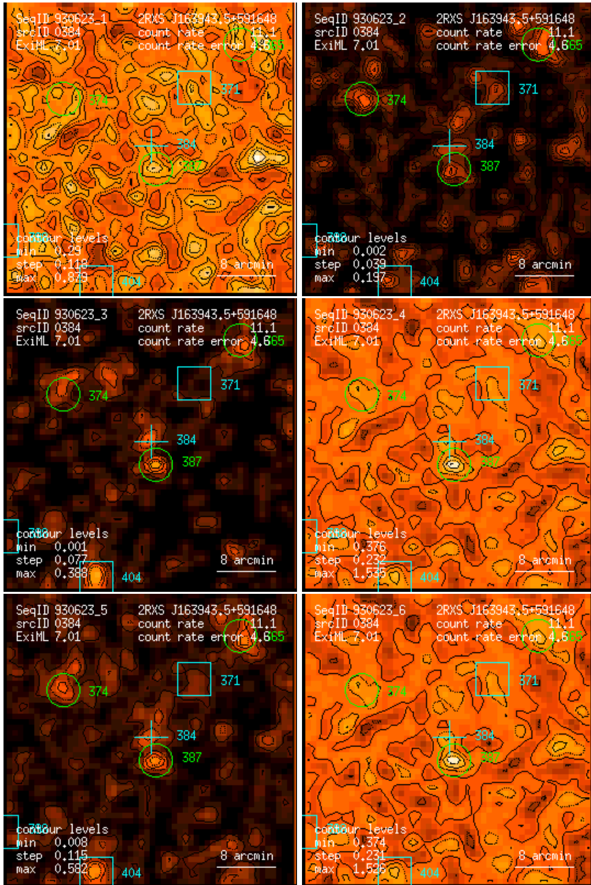
Figure 384: RASS 930623: detection 0384: band rate images, Gaussian filter: (1) PSPC channels 11 – 41, (2) 52 – 90, (3) 91 – 201, (4) 11 – 235, (5) 52 – 201, (6) 11 – 201. Broad band rates in counts/ks. Band rate contour levels in counts/ks/arcmin 2 .
