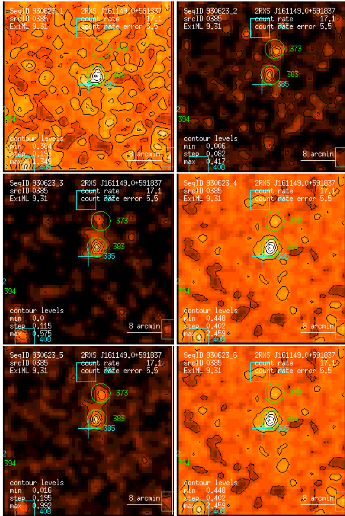
Figure 385: RASS 930623: detection 0385: band rate images, Gaussian filter: (1) PSPC channels 11 – 41, (2) 52 – 90, (3) 91 – 201, (4) 11 – 235, (5) 52 – 201, (6) 11 – 201. Broad band rates in counts/ks. Band rate contour levels in counts/ks/arcmin 2 .
