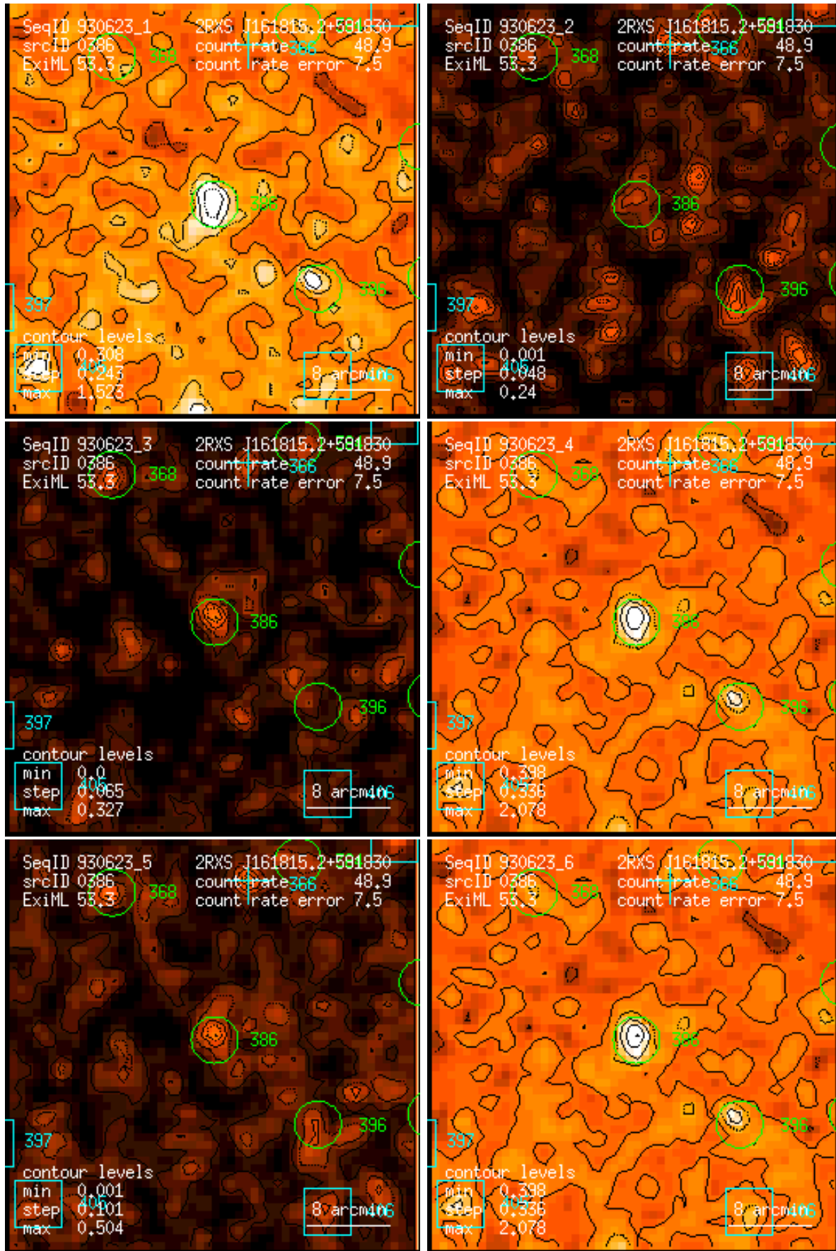
Figure 386: RASS 930623: detection 0386: band rate images, Gaussian filter: (1) PSPC channels 11 – 41, (2) 52 – 90, (3) 91 – 201, (4) 11 – 235, (5) 52 – 201, (6) 11 – 201. Broad band rates in counts/ks. Band rate contour levels in counts/ks/arcmin 2 .
