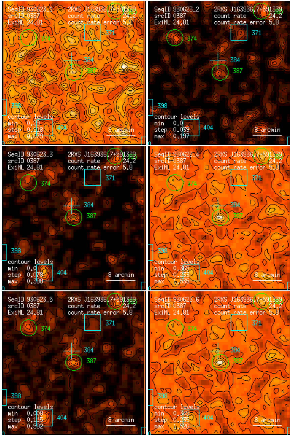
Figure 387: RASS 930623: detection 0387: band rate images, Gaussian filter: (1) PSPC channels 11 – 41, (2) 52 – 90, (3) 91 – 201, (4) 11 – 235, (5) 52 – 201, (6) 11 – 201. Broad band rates in counts/ks. Band rate contour levels in counts/ks/arcmin 2 .
