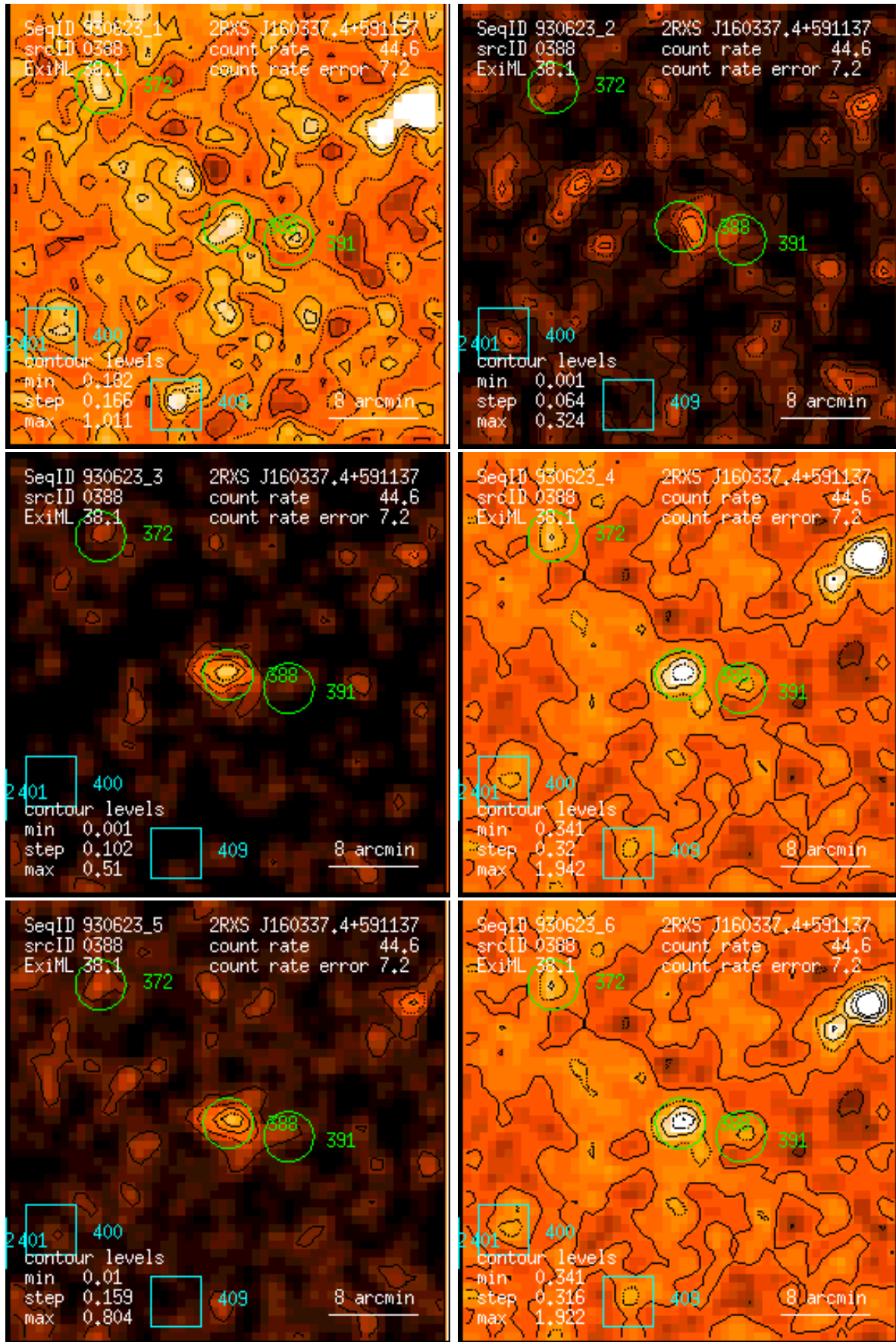
Figure 388: RASS 930623: detection 0388: band rate images, Gaussian filter: (1) PSPC channels 11 – 41, (2) 52 – 90, (3) 91 – 201, (4) 11 – 235, (5) 52 – 201, (6) 11 – 201. Broad band rates in counts/ks. Band rate contour levels in counts/ks/arcmin 2 .
