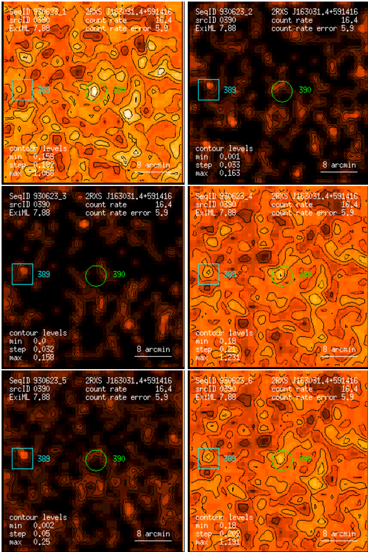
Figure 390: RASS 930623: detection 0390: band rate images, Gaussian filter: (1) PSPC channels 11 – 41, (2) 52 – 90, (3) 91 – 201, (4) 11 – 235, (5) 52 – 201, (6) 11 – 201. Broad band rates in counts/ks. Band rate contour levels in counts/ks/arcmin 2 .
